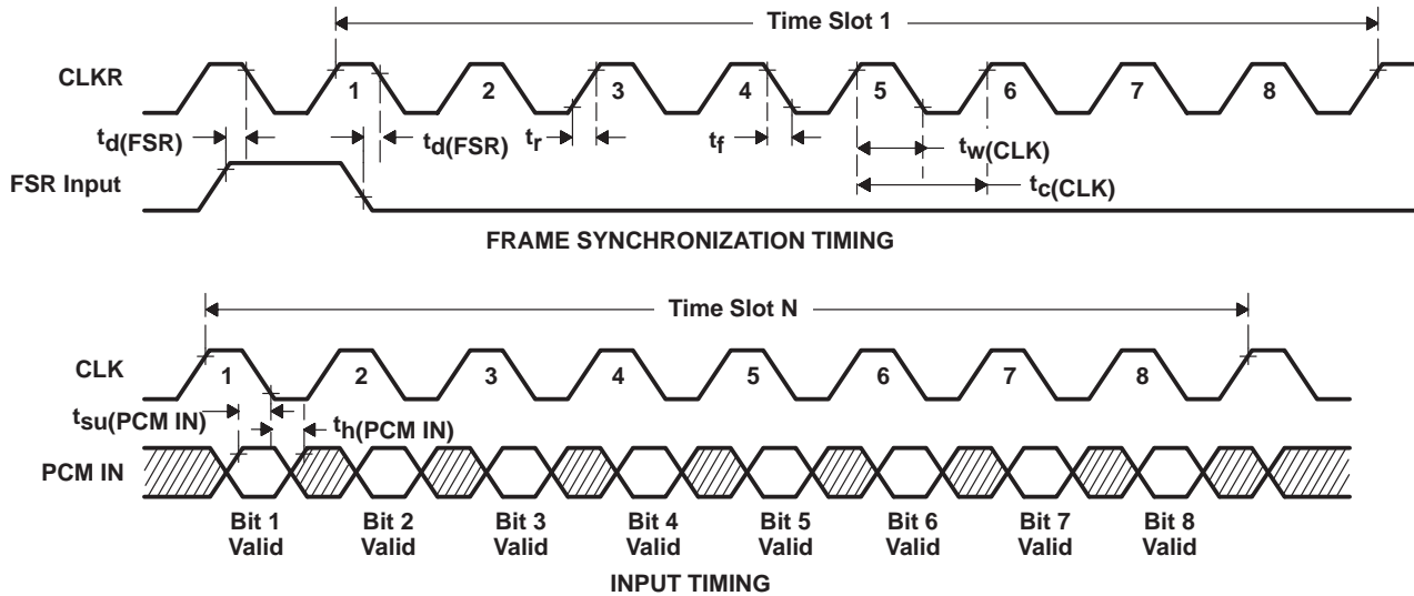
Figure 3. Transmit Timing (Fixed-Data Rate)
