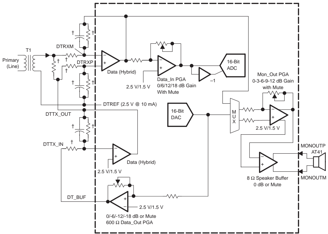
Figure 6–3. Data Channel Codec Typical Application
