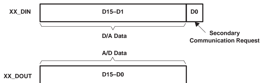
Figure 4–1. Primary Communication DIN and DOUT Data Format
