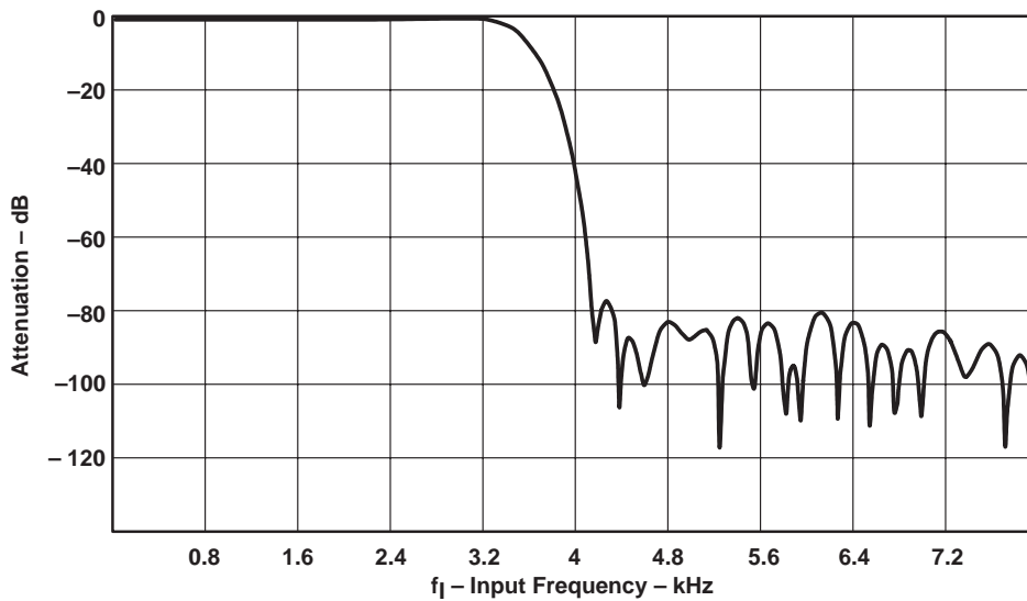
Figure 5–2. ADC Decimation Filter Response
