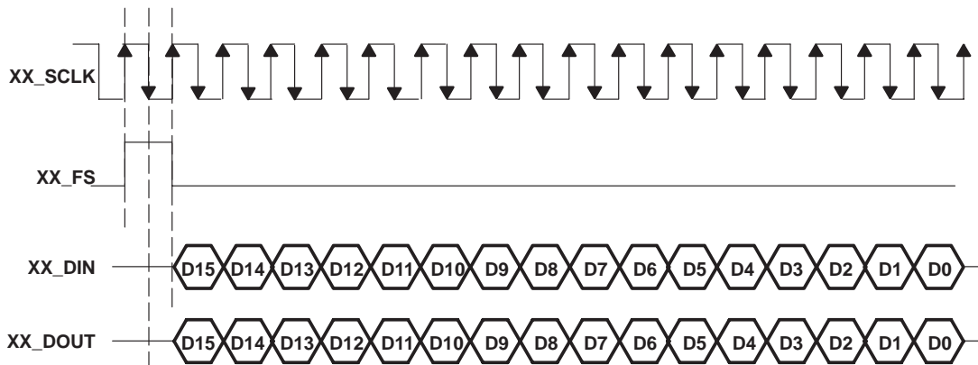
Figure 4–2. FS High Mode Primary Serial Communication Timing
