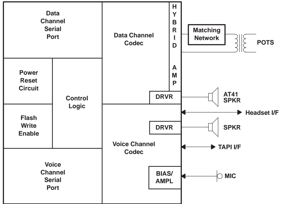
Figure 6–1. Functional Block of a Typical Application
