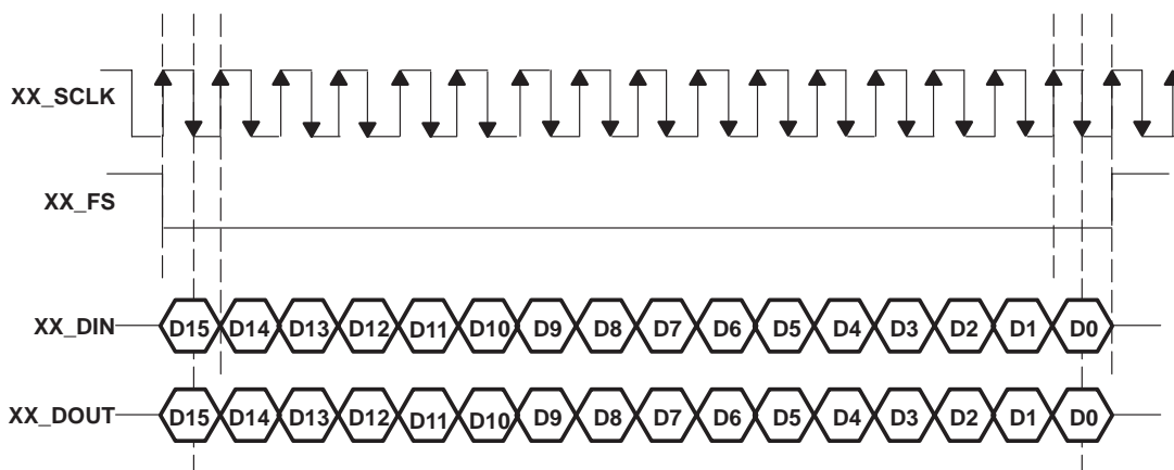
Figure 4–3. FS Low Mode Primary Serial Communication Timing
