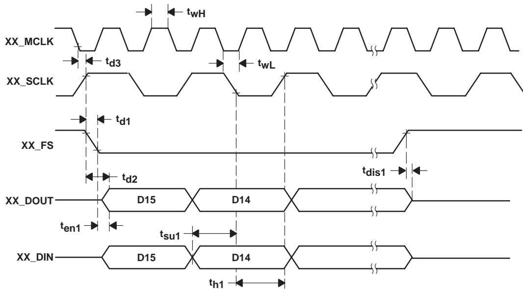
Figure 5–1. Serial Communication Timing for FS High Mode
