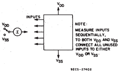
Fig. 13 - Input current.
