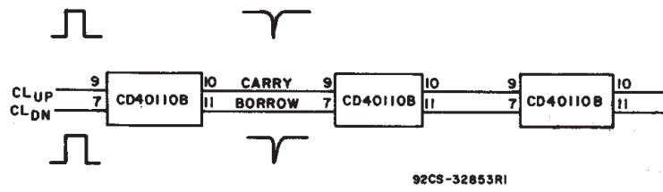
Fig. 15 - Cascading diagram.
