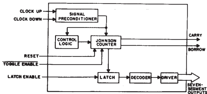
Fig. 1 - Functional diagram.
