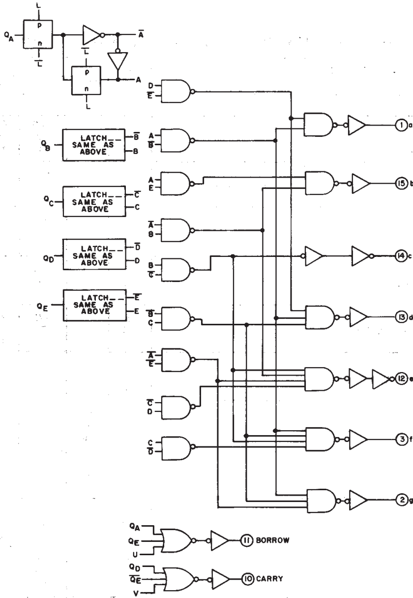
Fig. 2 - Logic diagram with flip-flop and output-driver details.
