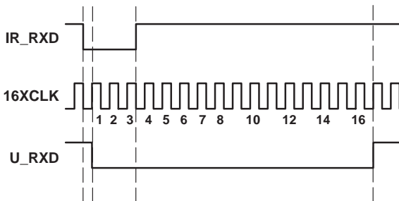
Figure 4. IrDA-SIR Decoding Scheme – Detailed Timing Diagram
