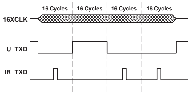
Figure 3. Encoding Scheme – Macro View
