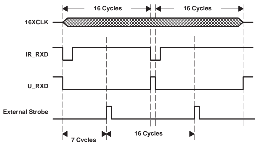
Figure 7. Recommended Strobing For Decoded Data
