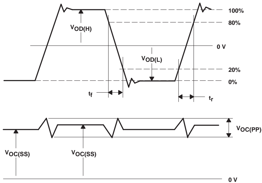
(b) WAVEFORMS
