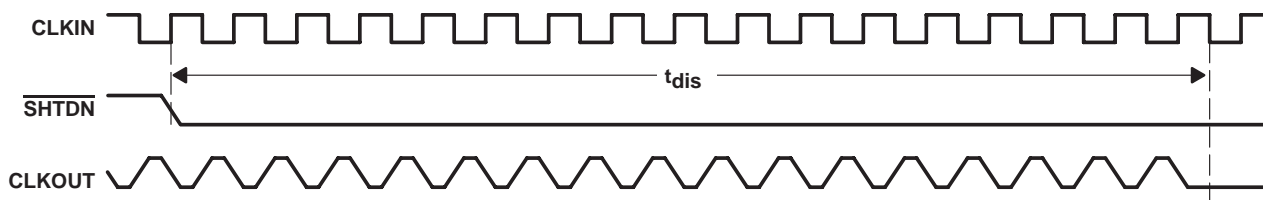
Figure 9. Disable Time Waveforms
