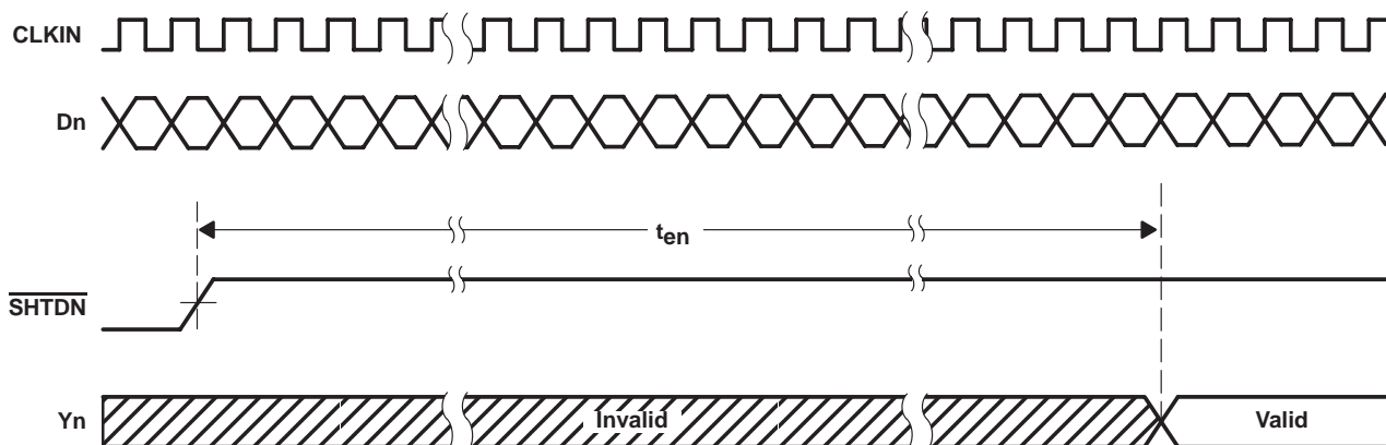
Figure 8. Enable Time Waveforms
