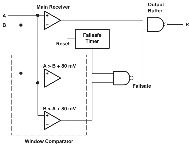
Figure 11. Receiver with Terminated Failsafe
