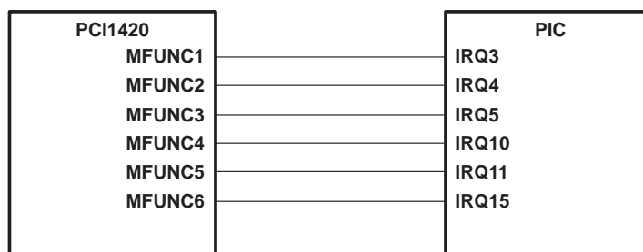
Figure 3–17. IRQ Implementation
