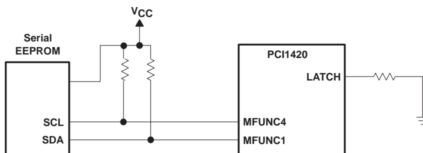
Figure 3–9. Serial EEPROM Application
