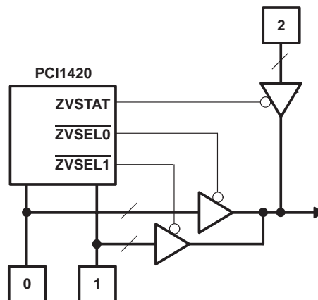
Figure 3–6. Zoomed Video Switching Application
