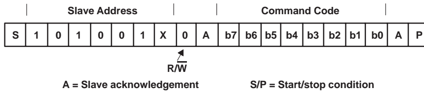
Figure 3–16. Send Byte Protocol
