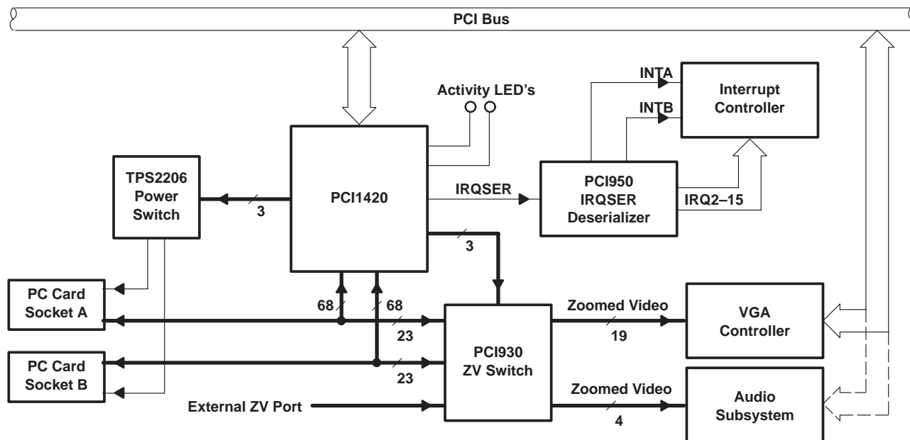
Figure 3–1. PCI1420 Simplified Block Diagram
