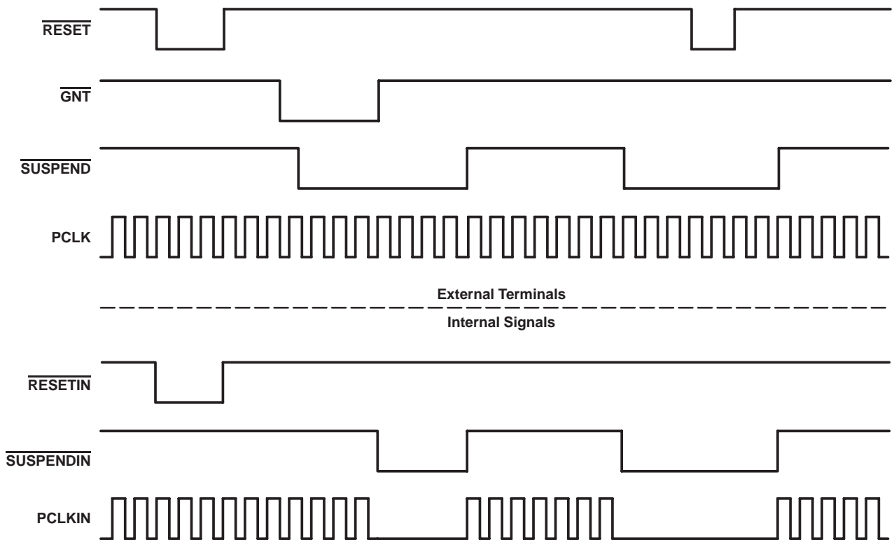
Figure 3–19. Signal Diagram of Suspend Function
