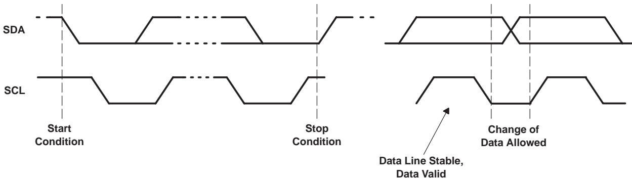
Figure 3–10. Serial Bus Start/Stop Conditions and Bit Transfers
