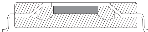
Figure 9. Leadframe Downset
