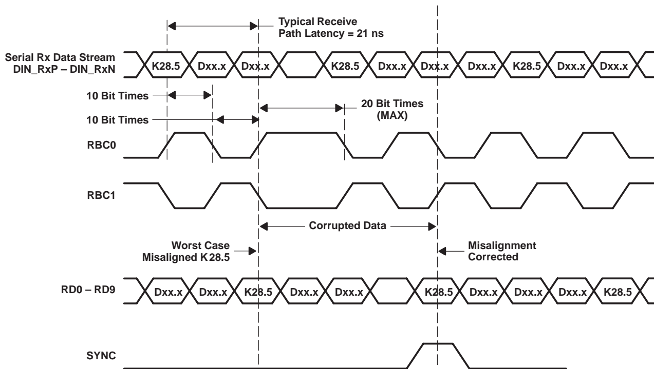
Figure 2. Word Realignment Timing Characteristics Waveforms
