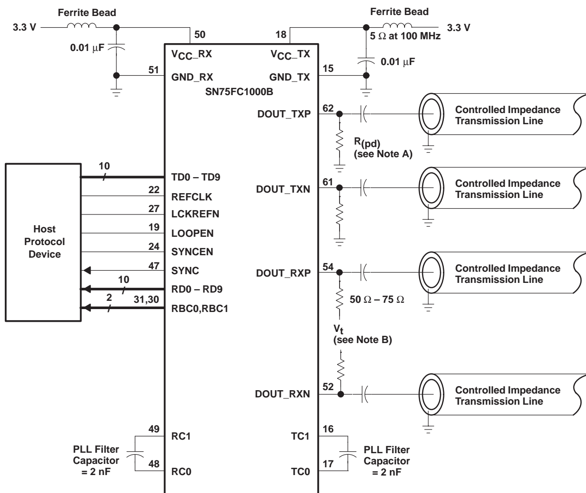
Figure 7. Typical Application Circuit
