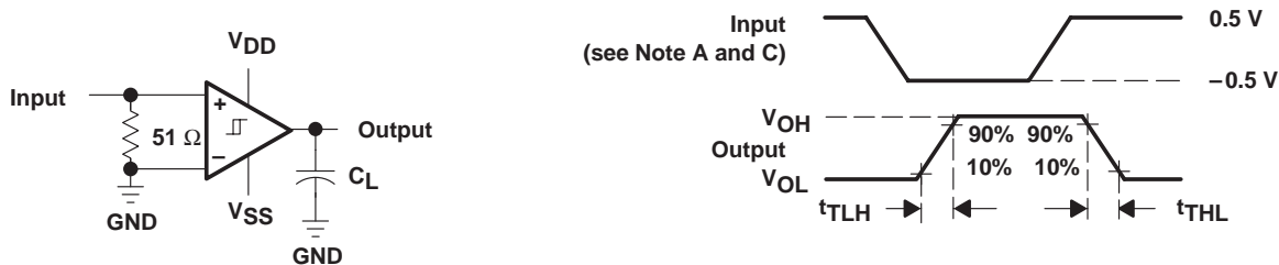
Figure 3. Receiver Transition Times
