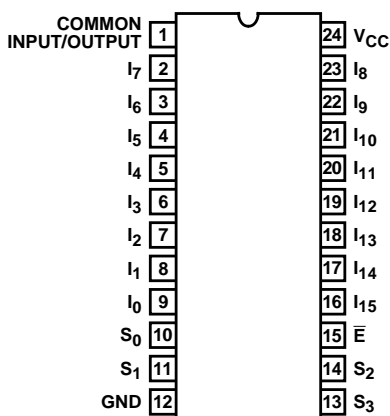
CD74HC4067, CD74HCT4067 (PDIP, SOIC) TOP VIEW
