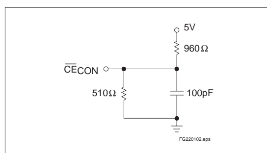
Figure 3. Output Load
