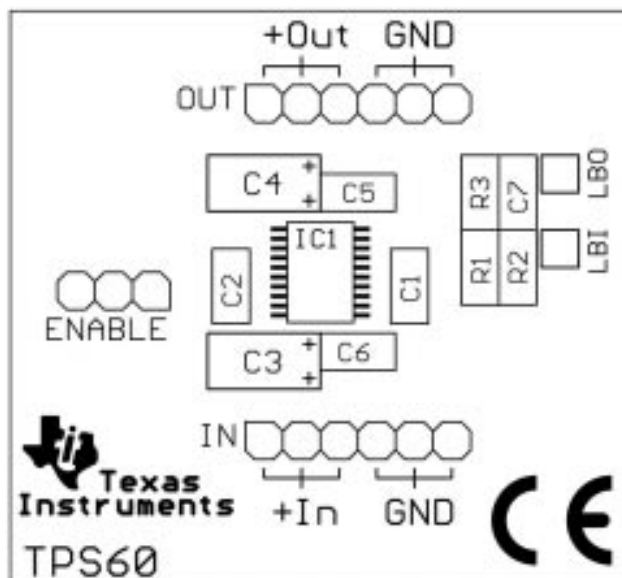
Figure 24. Component Placement
