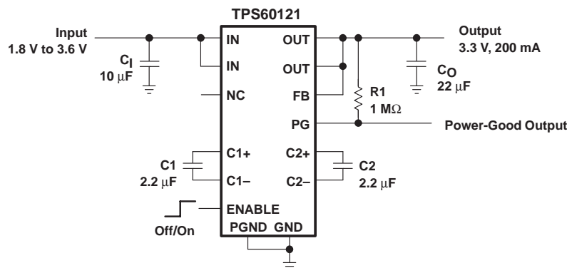
Figure 2. Typical Operating Circuit Using Power-Good Comparator
