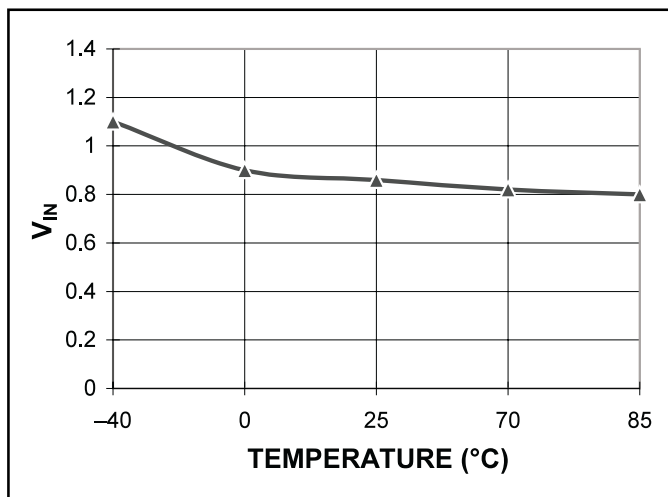
Figure 15. V_{IN} startup vs. temp.
