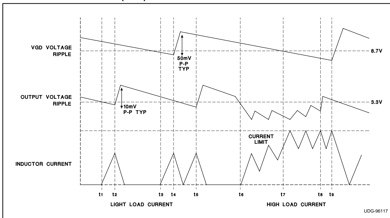
Figure 2. Inductor current and output ripple waveforms.
