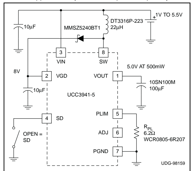
Figure 4. Dual output synchronous boost 5V version.
