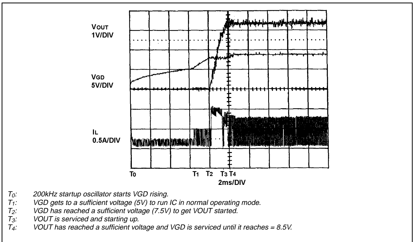
Figure 8. Startup characteristics.
