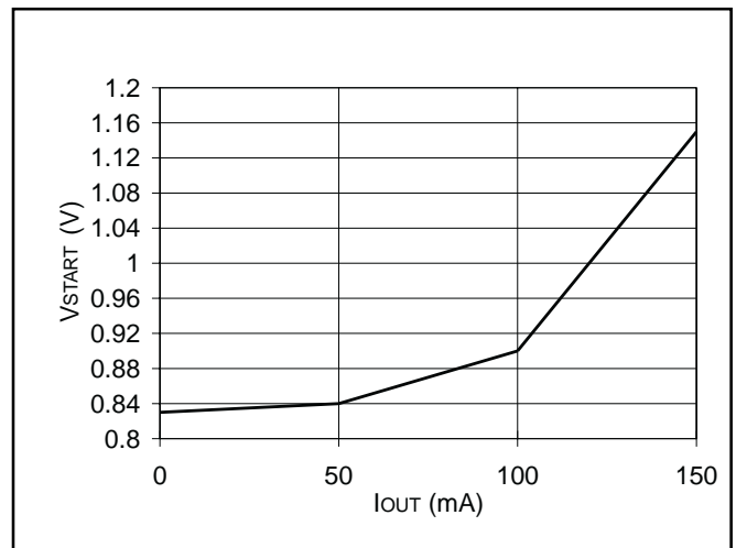
Figure 12. Minimum start voltage vs. I_{OUT} .
