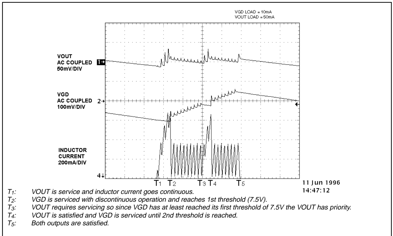
Figure 9. Dual output example.
