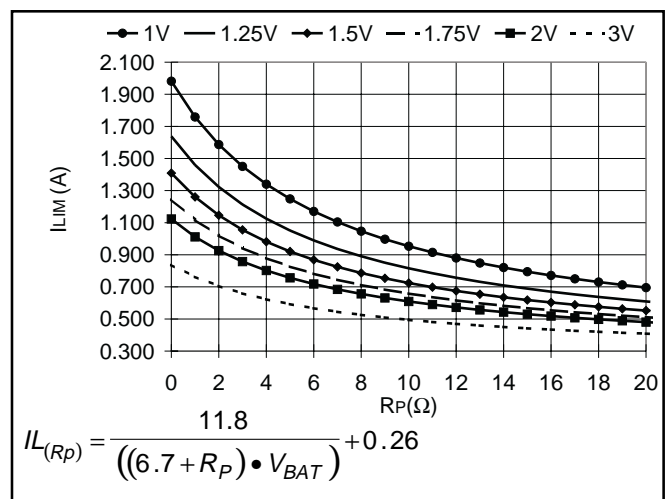
Figure 14. UCC3941-ADJ I_{LIM} vs. R_P (all other packages).
