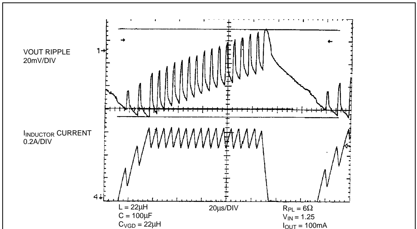
Figure 10. Pseudo continuous mode operation.
