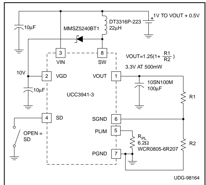
Figure 5. Dual output synchronous boost ADJ version.
