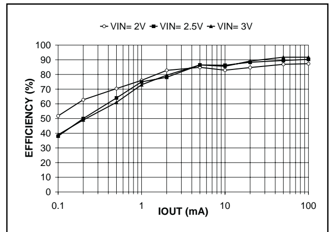
Figure 7. UCC3941 Efficiency vs. I_{OUT} , V_{OUT} = 3.3V .
