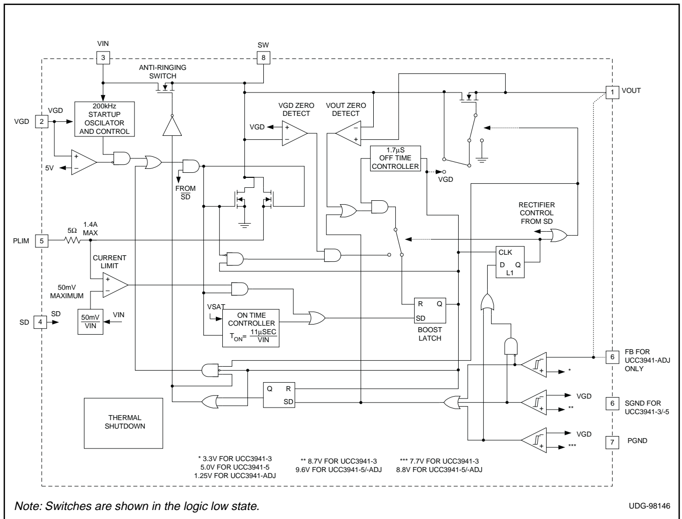
Figure 1. 1V Synchronous boost.
