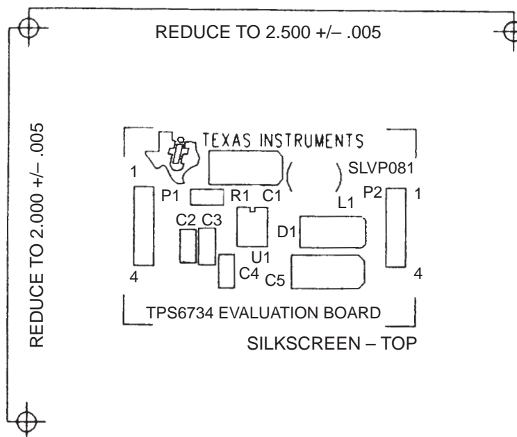
Figure 14. Component Placement
