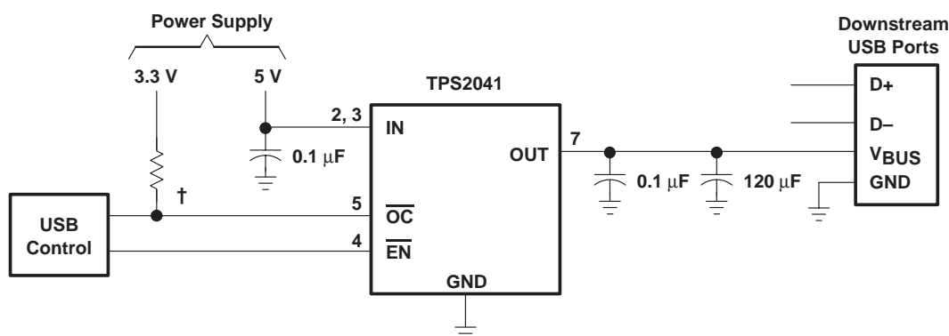
Figure 31. One-Port Solution
