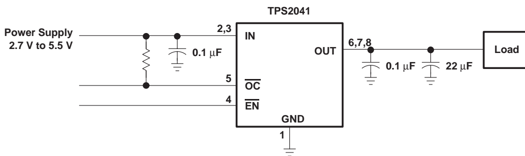
Figure 29. Typical Application
