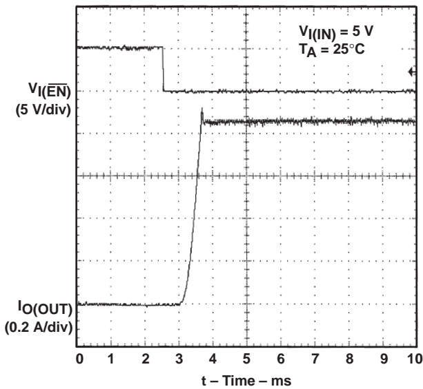
Figure 6. TPS2041, Short-Circuit Current, Device Enabled into Short
