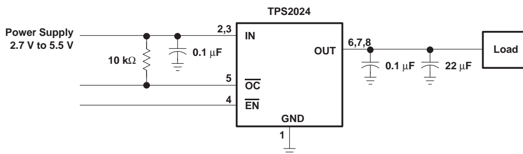
Figure 38. Typical Application
