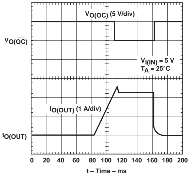
Figure 10. TPS2023, Ramped Load on Enabled Device
