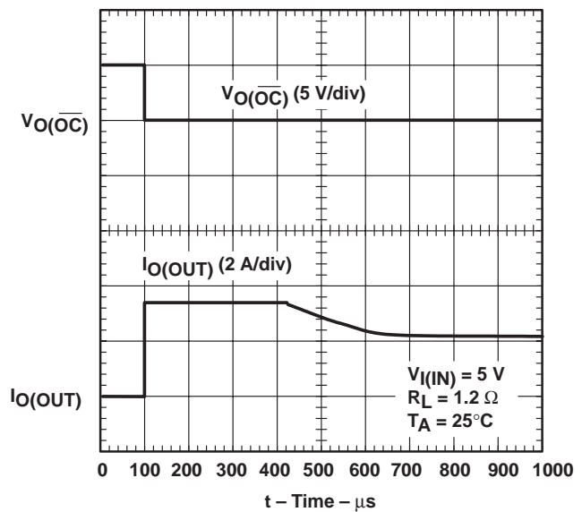
Figure 19. 1.2- \Omega Load Connected to an Enabled TPS2023 Device
