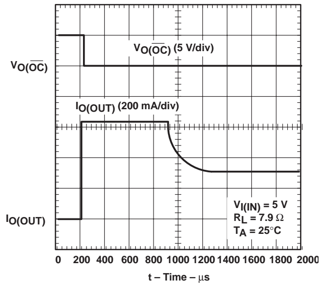
Figure 13. 7.9- \Omega Load Connected to an Enabled TPS2020 Device
