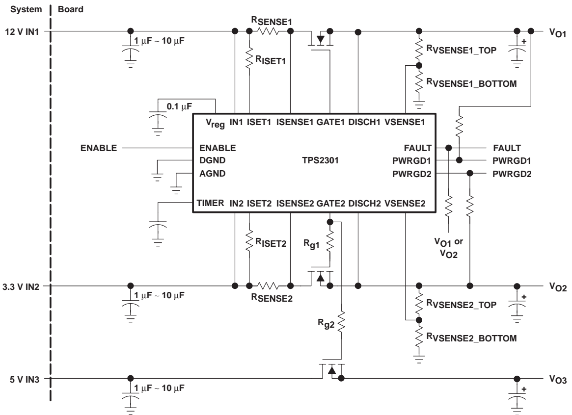
Figure 28. Three-Channel Application
