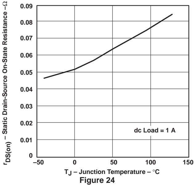
STATIC DRAIN-SOURCE ON-STATE RESISTANCE, 3.3-V xVCC SWITCH vs JUNCTION TEMPERATURE
