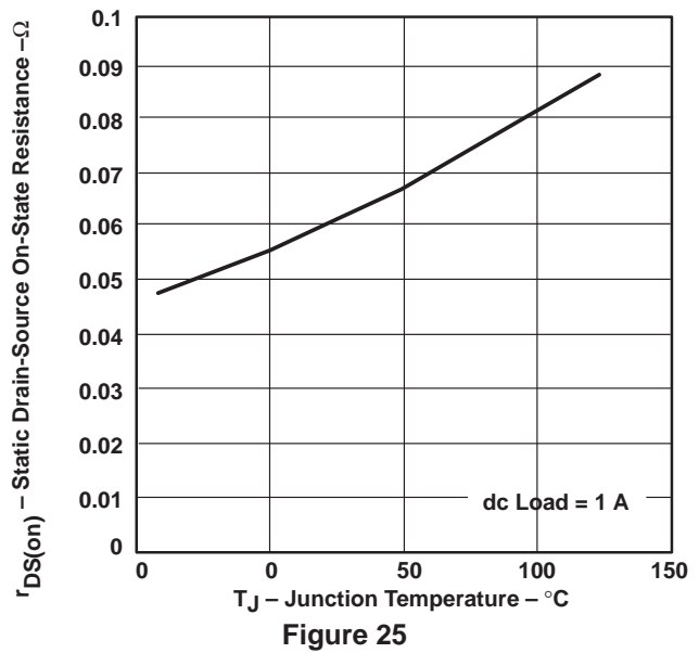
STATIC DRAIN-SOURCE ON-STATE RESISTANCE, 5-V xVCC SWITCH vs JUNCTION TEMPERATURE
