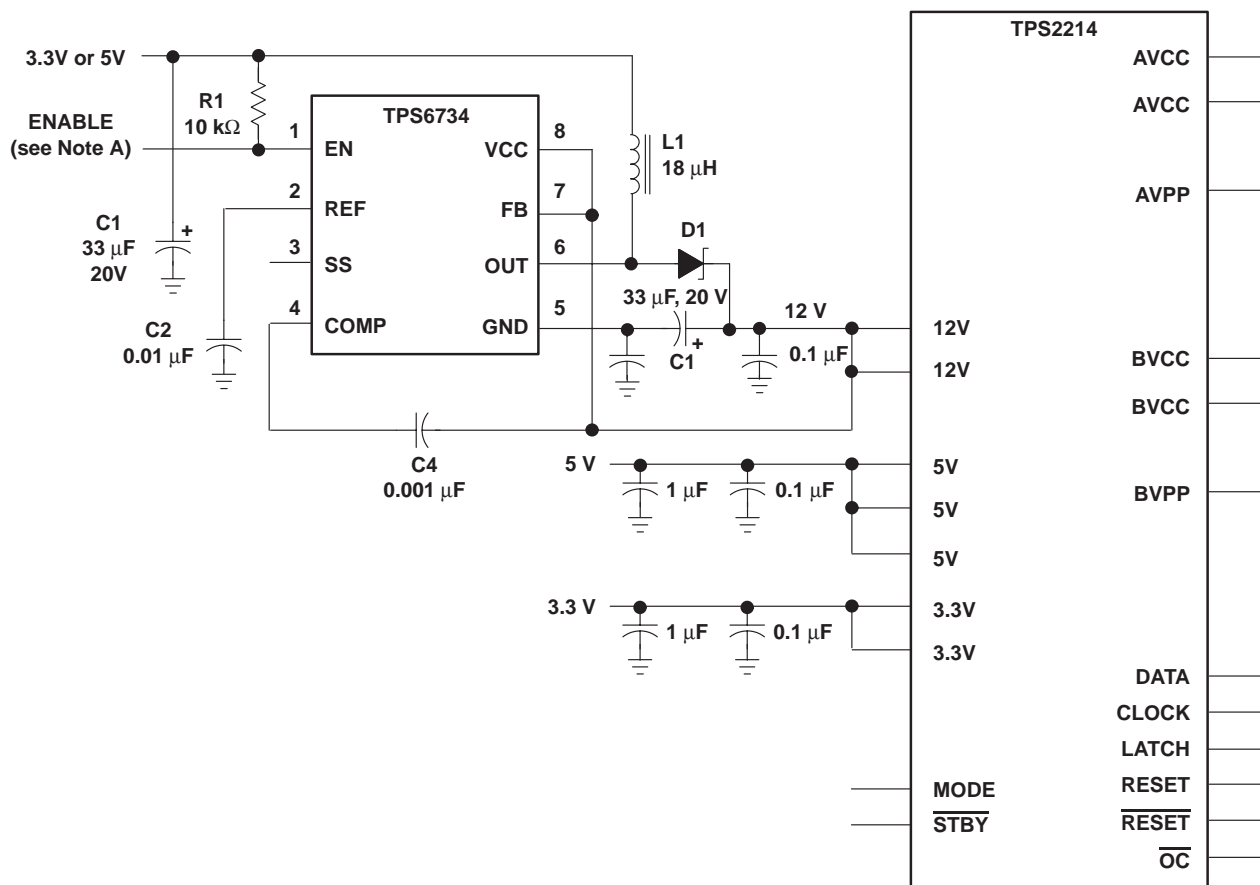
Figure 35. TPS2214 with TPS6734 12-V, 120-mA Supply
