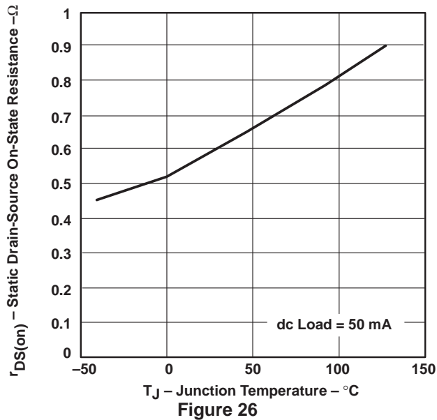
STATIC DRAIN-SOURCE ON-STATE RESISTANCE, 12-V xVPP SWITCH vs JUNCTION TEMPERATURE
