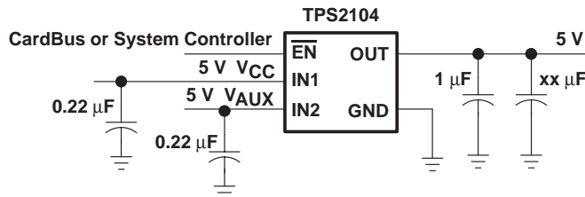
Figure 19. Typical Application
