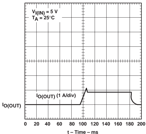
Figure 8. TPS2011A, Ramped Load on Enabled Device
