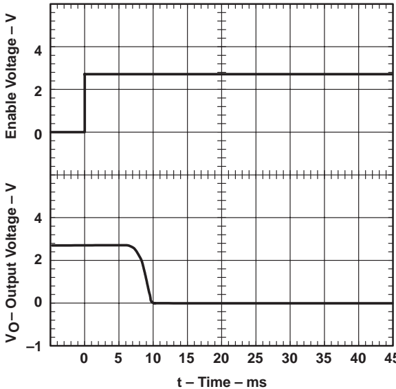
Figure 4. Propagation Delay and Fall Time With 1- \mu F Load, V_{I(IN)} = 2.7 V
