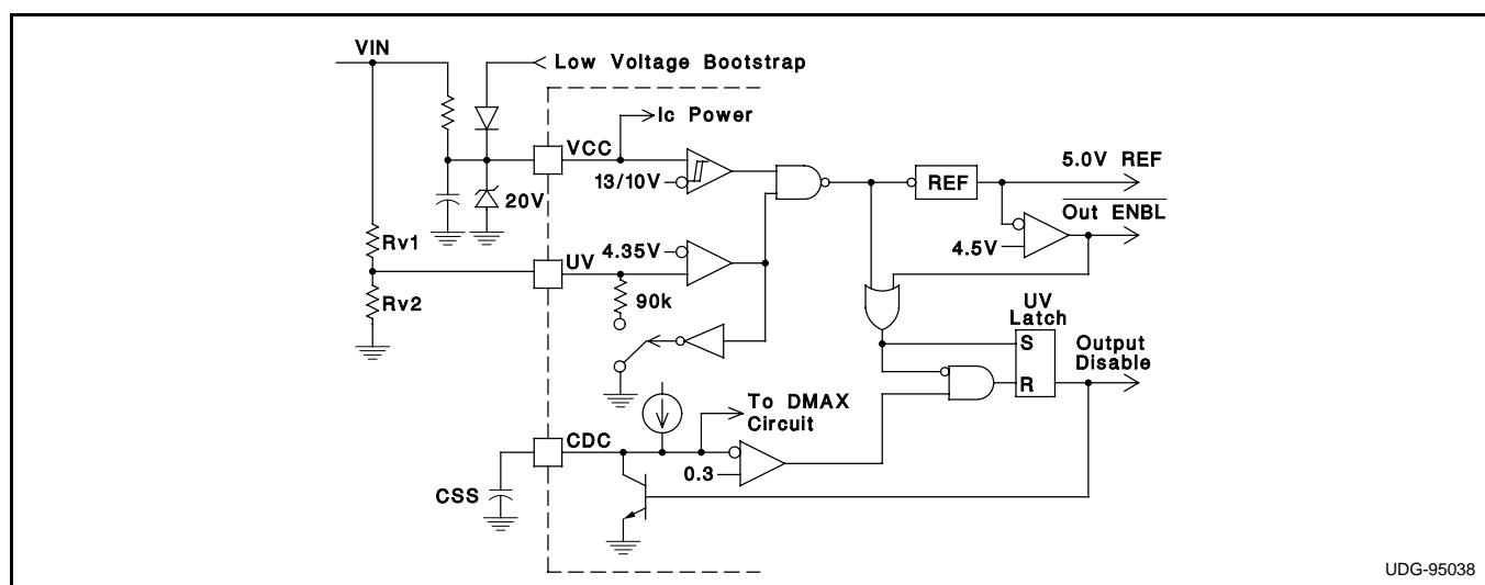
Figure 1: Undervoltage Lockout
