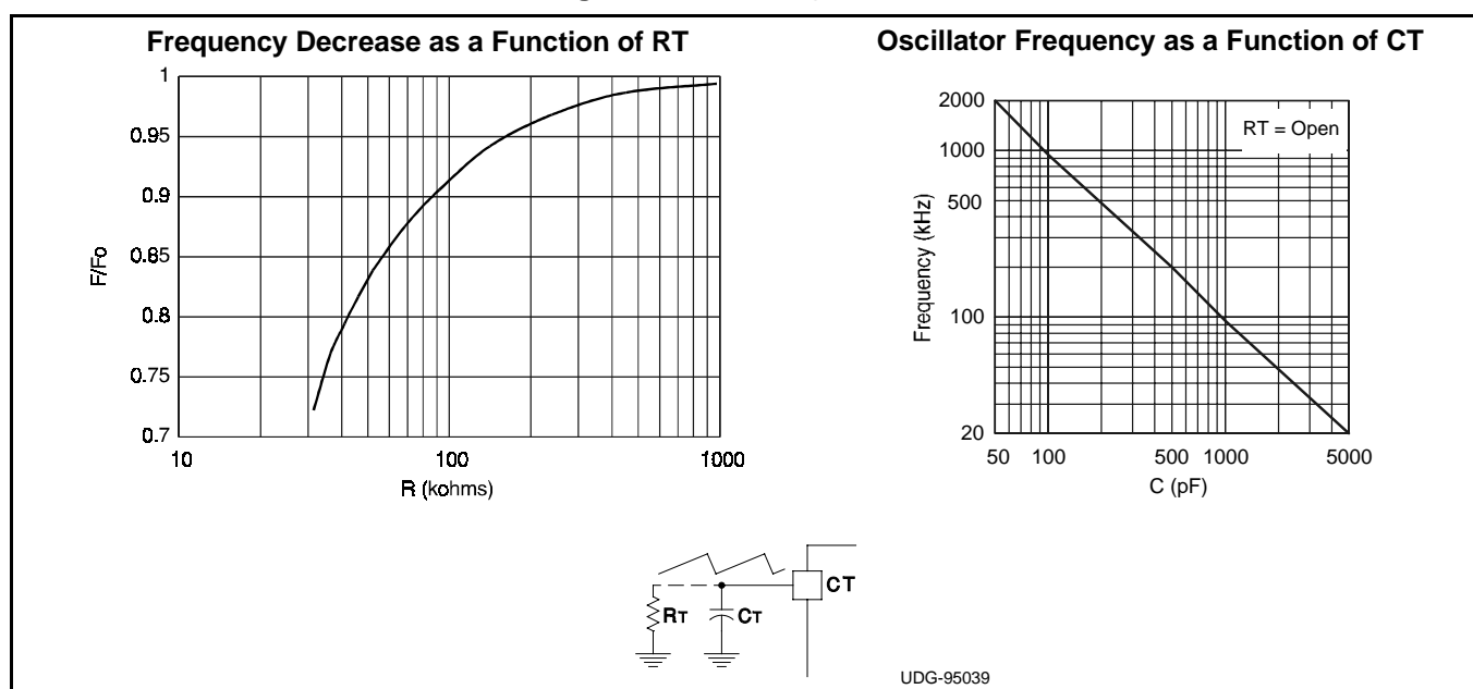
Figure 2: Oscillator Frequency
