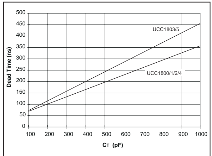
Figure 9. Dead time vs. C_T , R_T = 100k .
