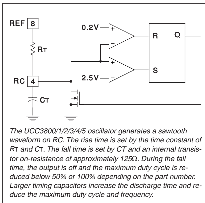
Figure 1. Oscillator.
