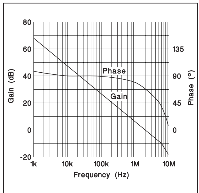
Figure 2. Error amplifier gain/phase response.
