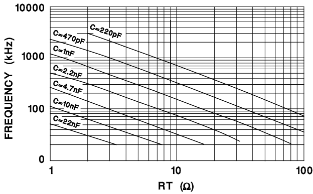
Oscillator Frequency vs. RT and CT Curve
