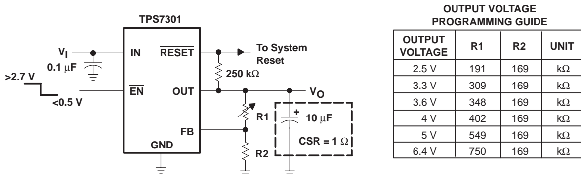
Figure 48. TPS7301 Adjustable LDO Regulator Programming
