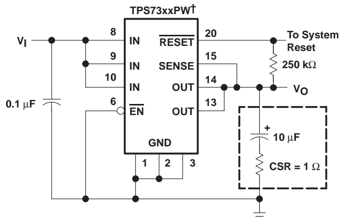
Figure 47. Typical Application Circuit
