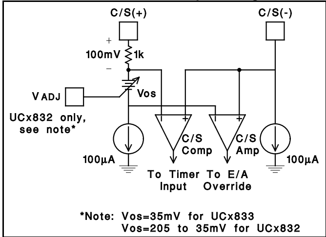
UCx832/33 Current Sense Input Configuration
