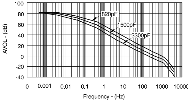
AVOL vs Frequency and CC
