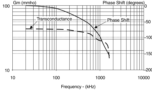
Transconductance and Phase vs Frequency
