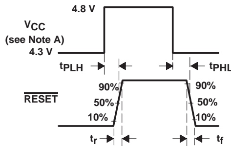
Figure 2. Switching Diagram
