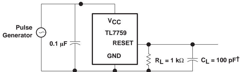
Figure 2. Switching Diagram
