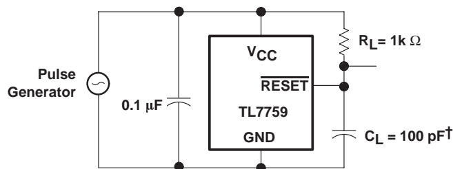
Figure 4. Test Circuit for \overline{\text{RESET}} Output Switching Characteristics
