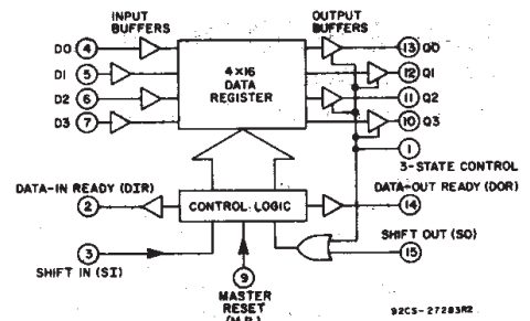
Fig. 2 - CD40105B functional block diagram.
