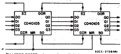
Fig. 3 - Expansion, 4-bits wide-by-16 N-bits long.
