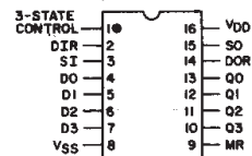
TERMINAL ASSIGNMENT
