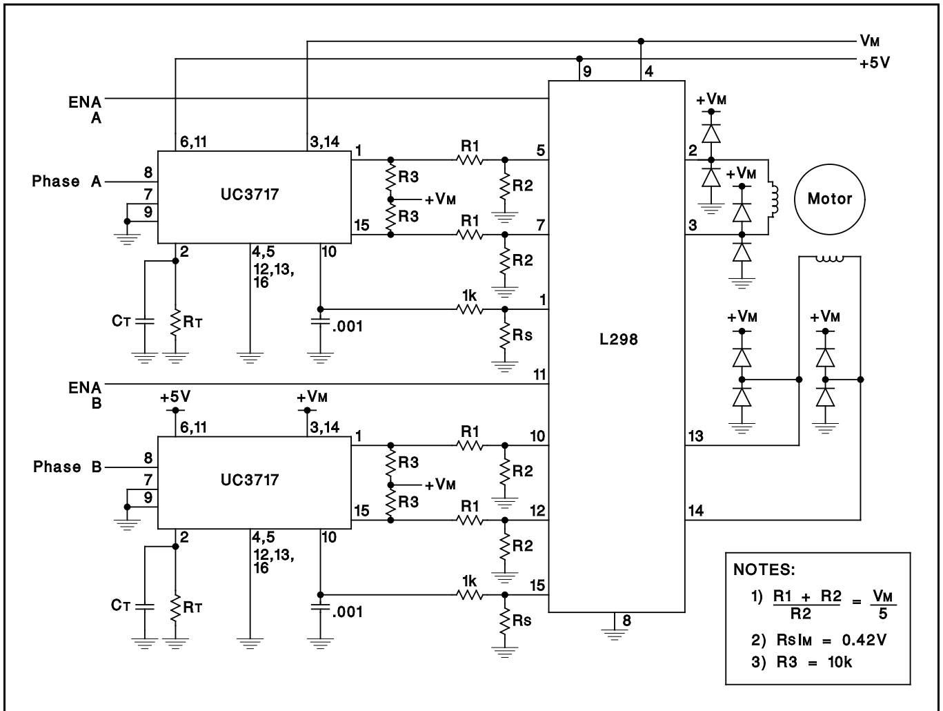
Figure 15: UC3717 with L298 Power Amplifier
