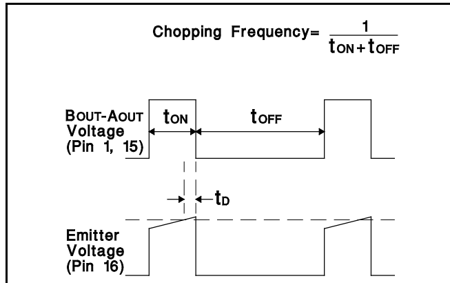
Figure 5: Connections and Component Values as in Figure 6.
