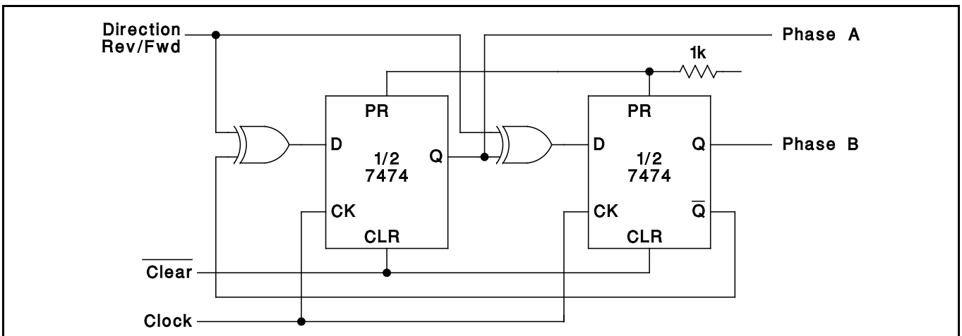
Figure 13: Full Step Bidirectional Two Phase Drive Logic
