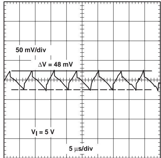
OUTPUT VOLTAGE RIPPLE
