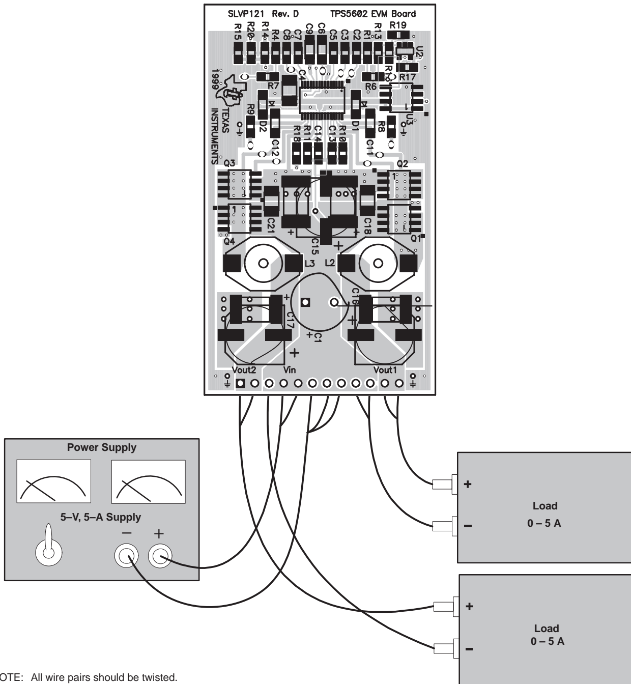
Figure 26. Test Setup
