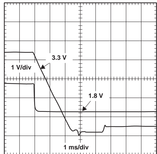
POWER-DOWN SEQUENCING
