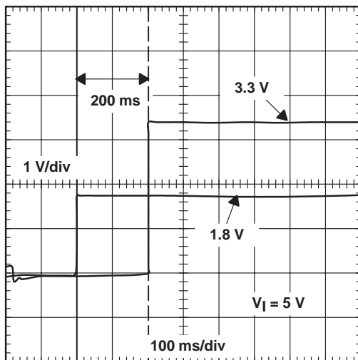
POWER-UP SEQUENCING
