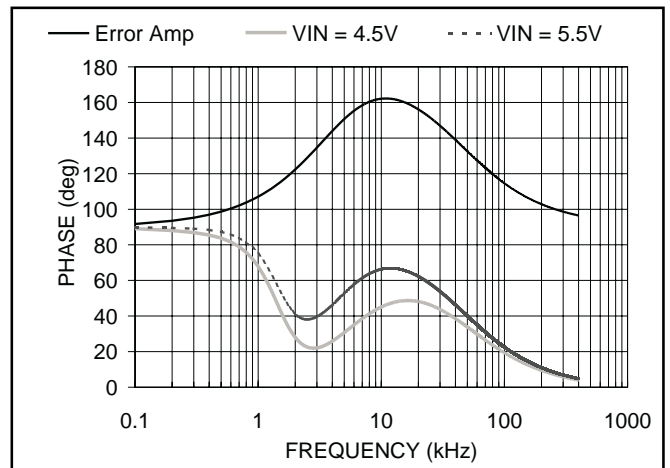
Figure 5. Error amplifier and loop frequency response.
