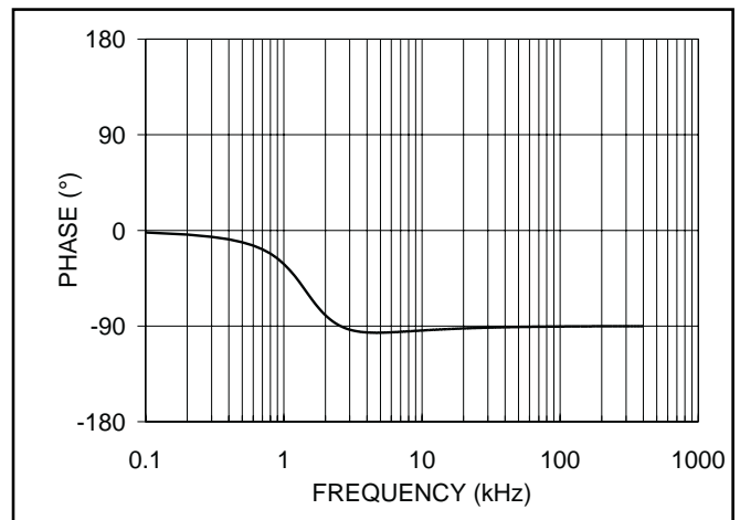
Figure 1. Modulator Frequency Response
