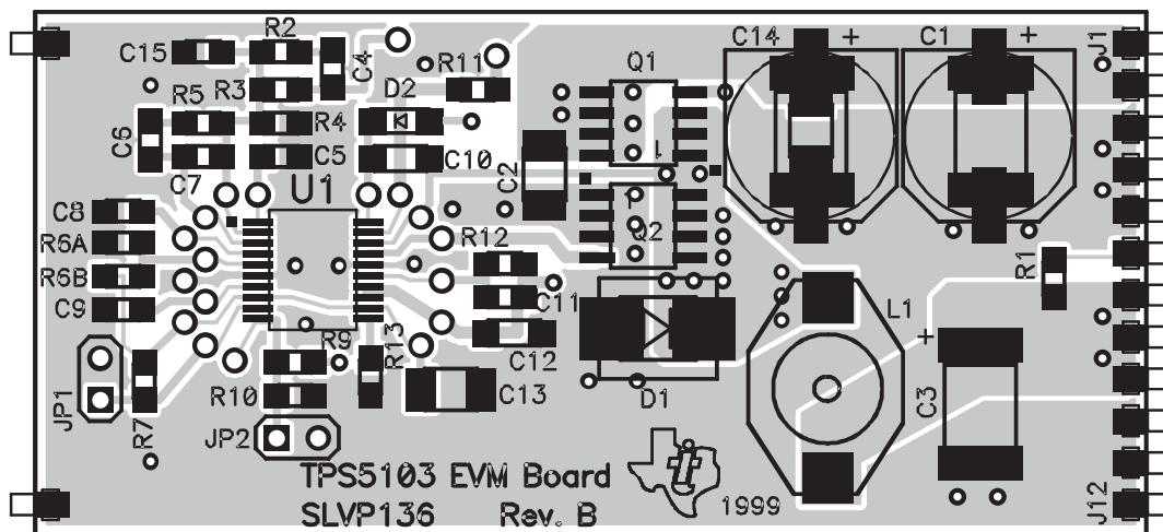
Top Assembly
