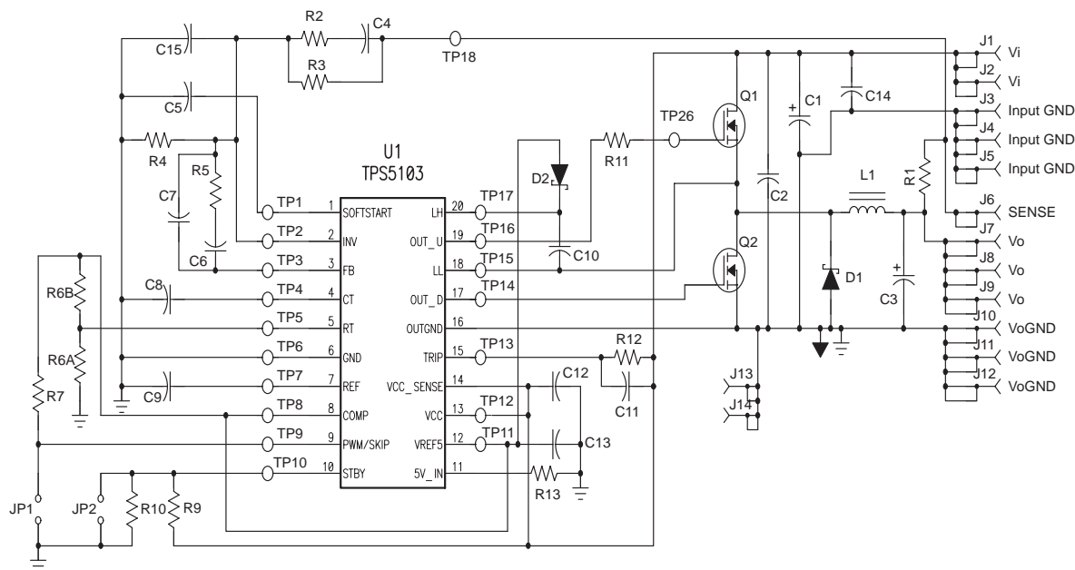
Figure 36. EVM Schematic
