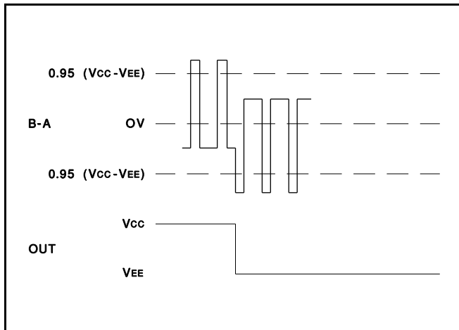
Figure 2. Input Waveform
