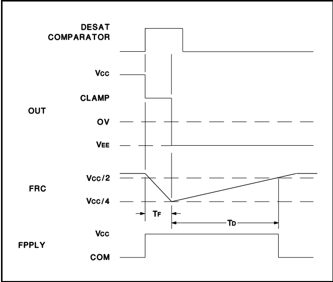
Figure 6. Desaturation Response
