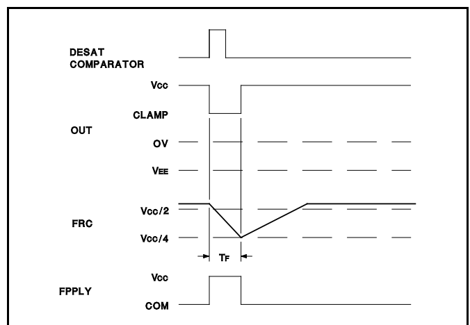
Figure 5. Transient Desaturation Response
