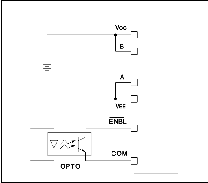
Figure 7. Using ENBL as Primary Input
