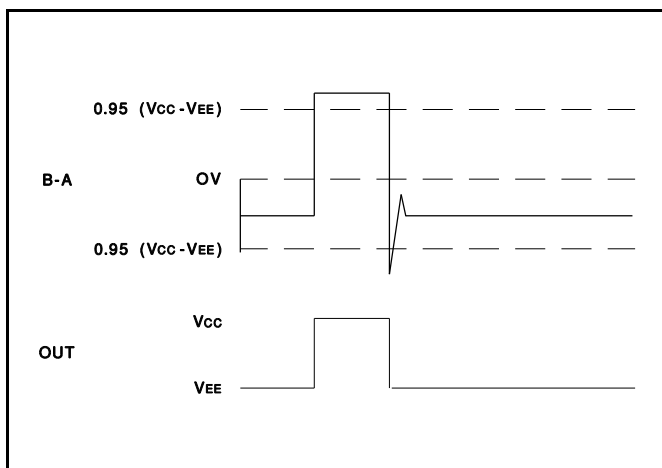
Figure 3. Output Pulsing Caused By Transformer Ringing
