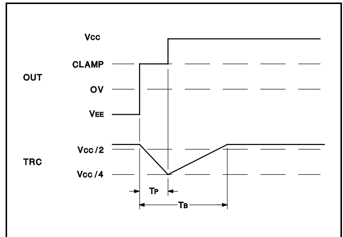
Figure 4. Rising Edge Waveform
