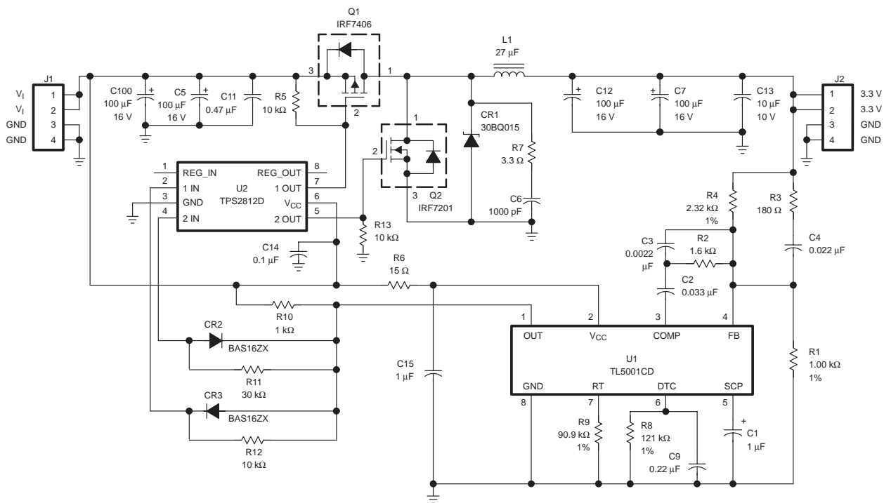
Figure 48. 3.3-V 3-A Synchronous-Rectified Buck Regulator Circuit
