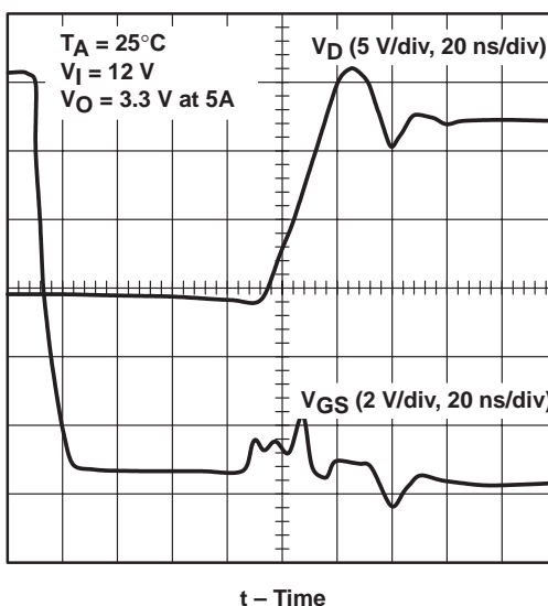
Figure 53. Q1 Drain Voltage vs Q2 Gate-Source Voltage
