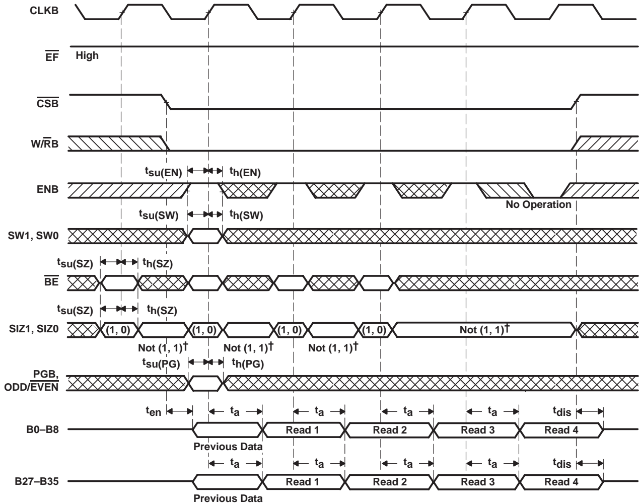
Figure 8. FIFO-Byte Read Cycle
