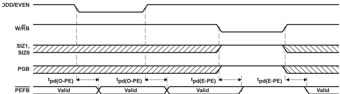
Figure 16. \overline{\text{ODD/EVEN}} , \overline{\text{W/RB}} , \overline{\text{SIZ1}} , \overline{\text{SIZ0}} , and \overline{\text{PGB}} to \overline{\text{PEFB}}
