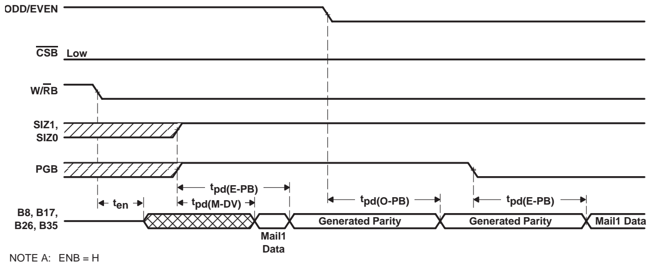
Figure 18. Parity Generation When Reading From the Mail1 Register
