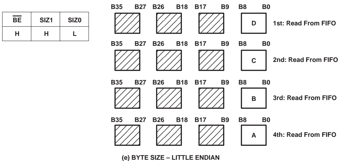
Figure 1. Dynamic Bus Sizing (Continued)
