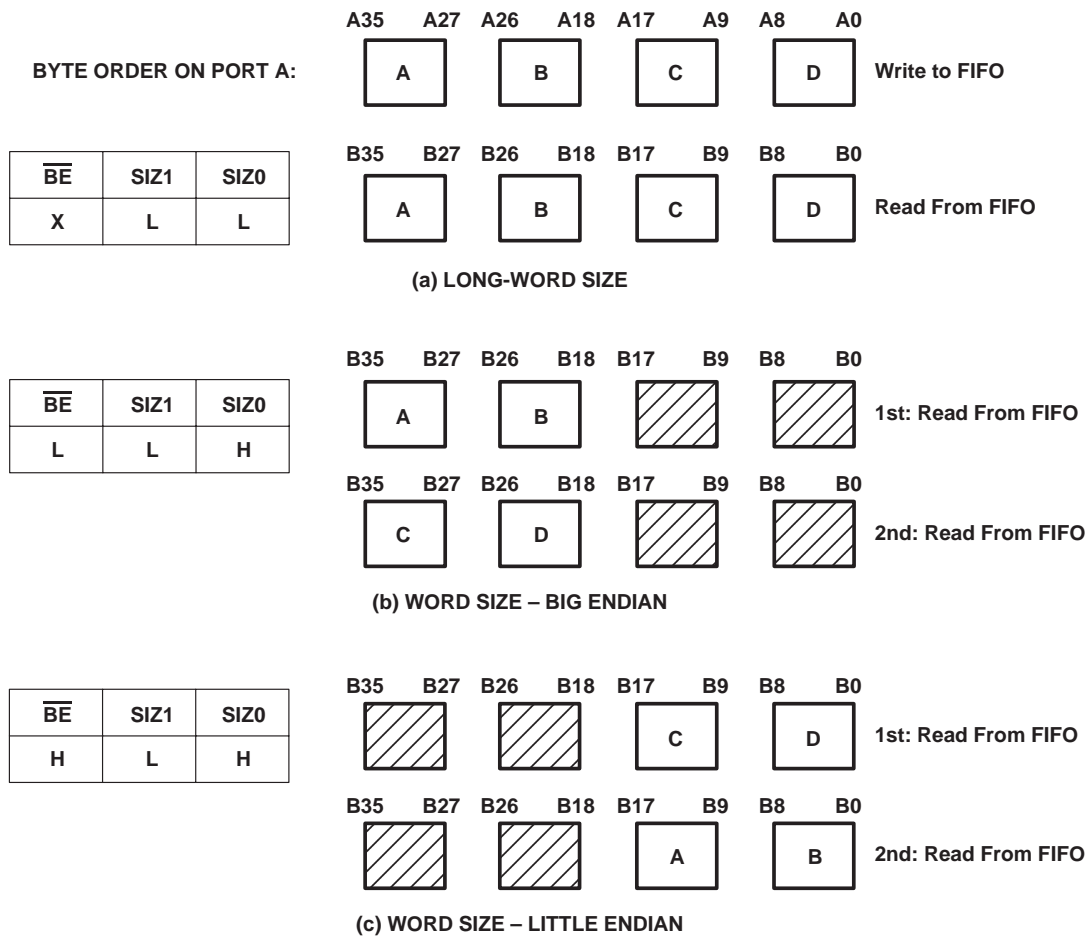
Figure 1. Dynamic Bus Sizing
