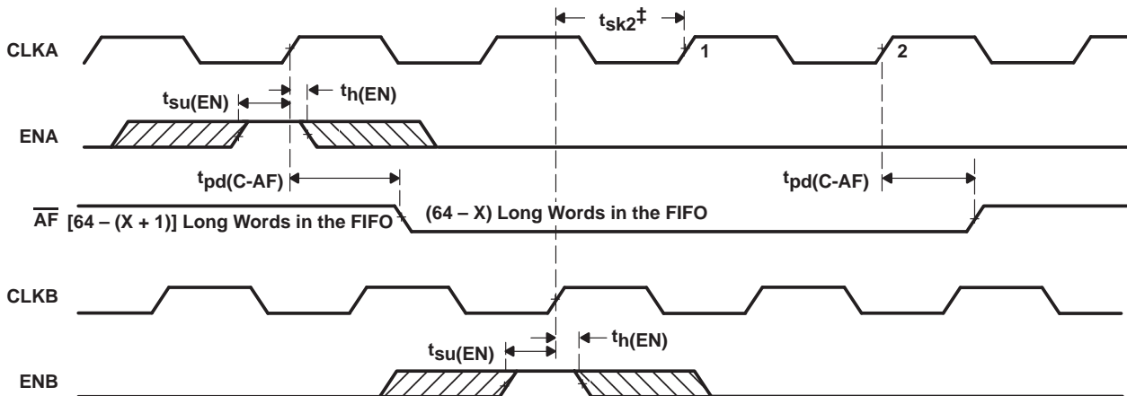
Figure 11. \overline{AE} When the FIFO Is Almost Empty
