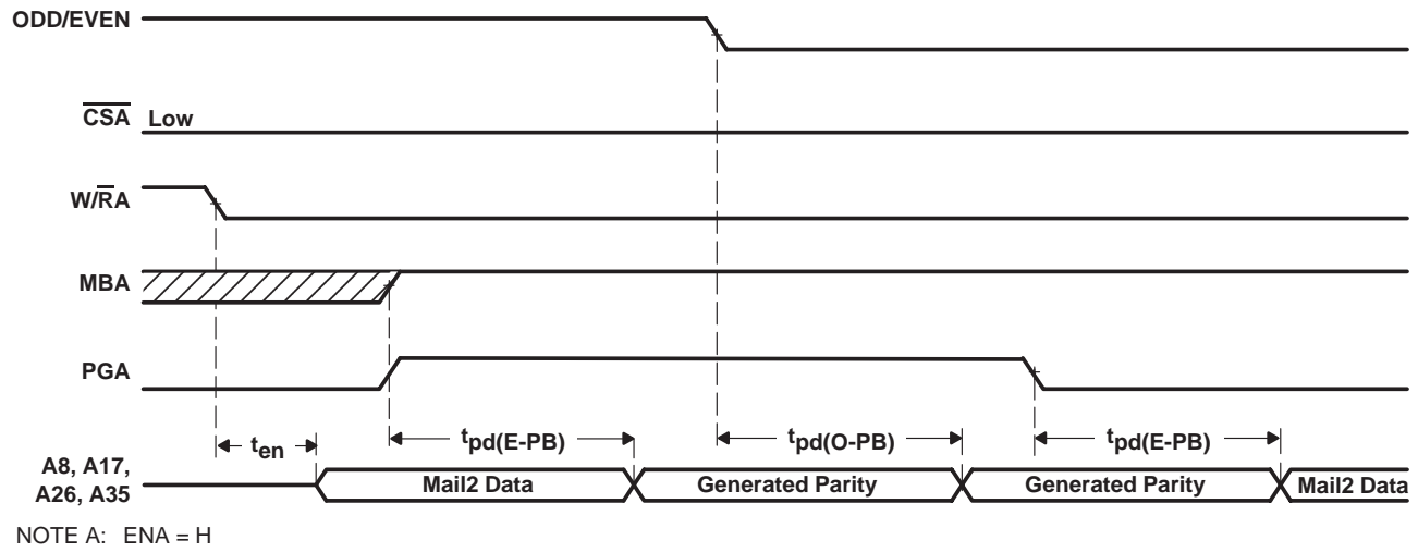
Figure 17. Parity Generation When Reading From the Mail2 Register
