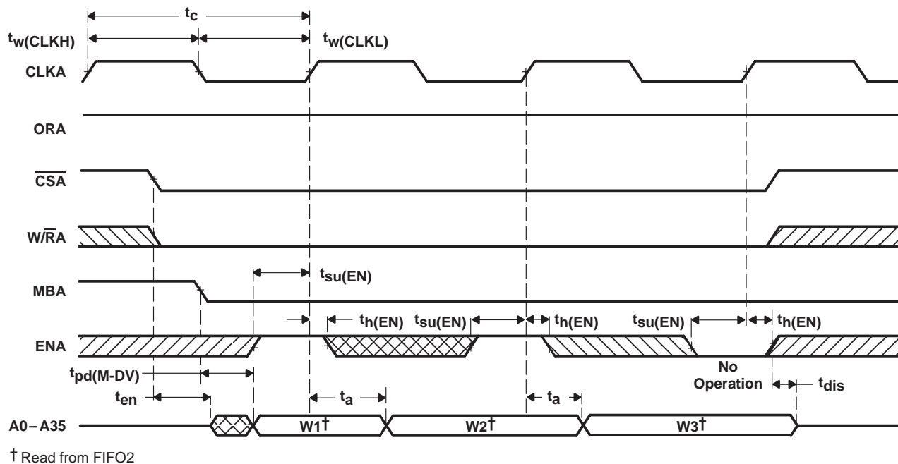
Figure 6. Port-A Read-Cycle Timing for FIFO2
