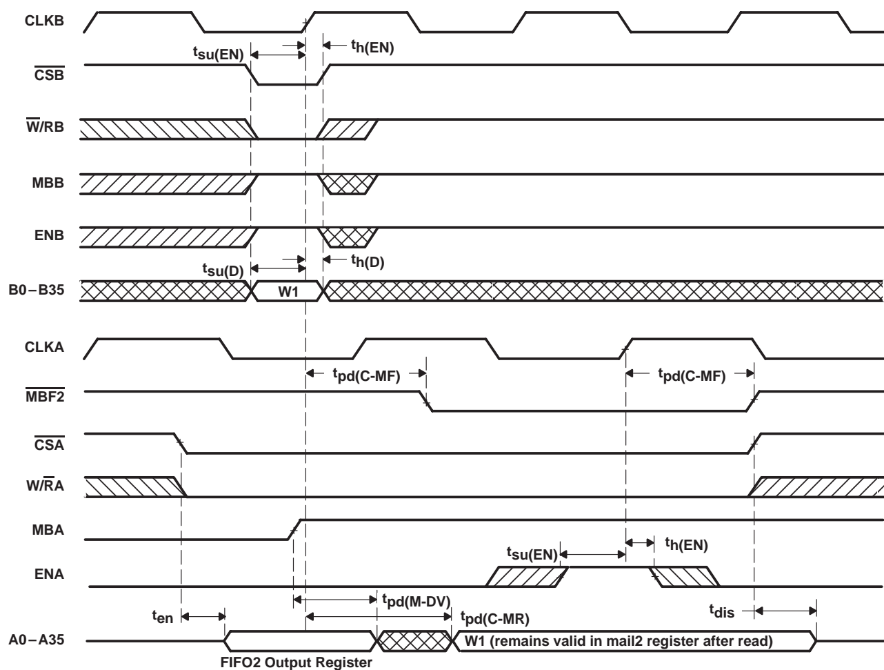
Figure 16. Timing for Mail2 Register and \overline{\text{MBF2}} Flag
