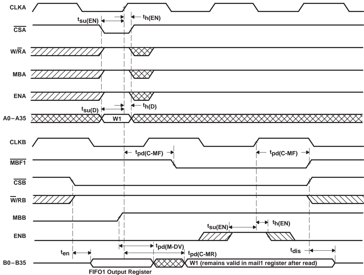
Figure 15. Timing for Mail1 Register and \overline{MBF1} Flag
