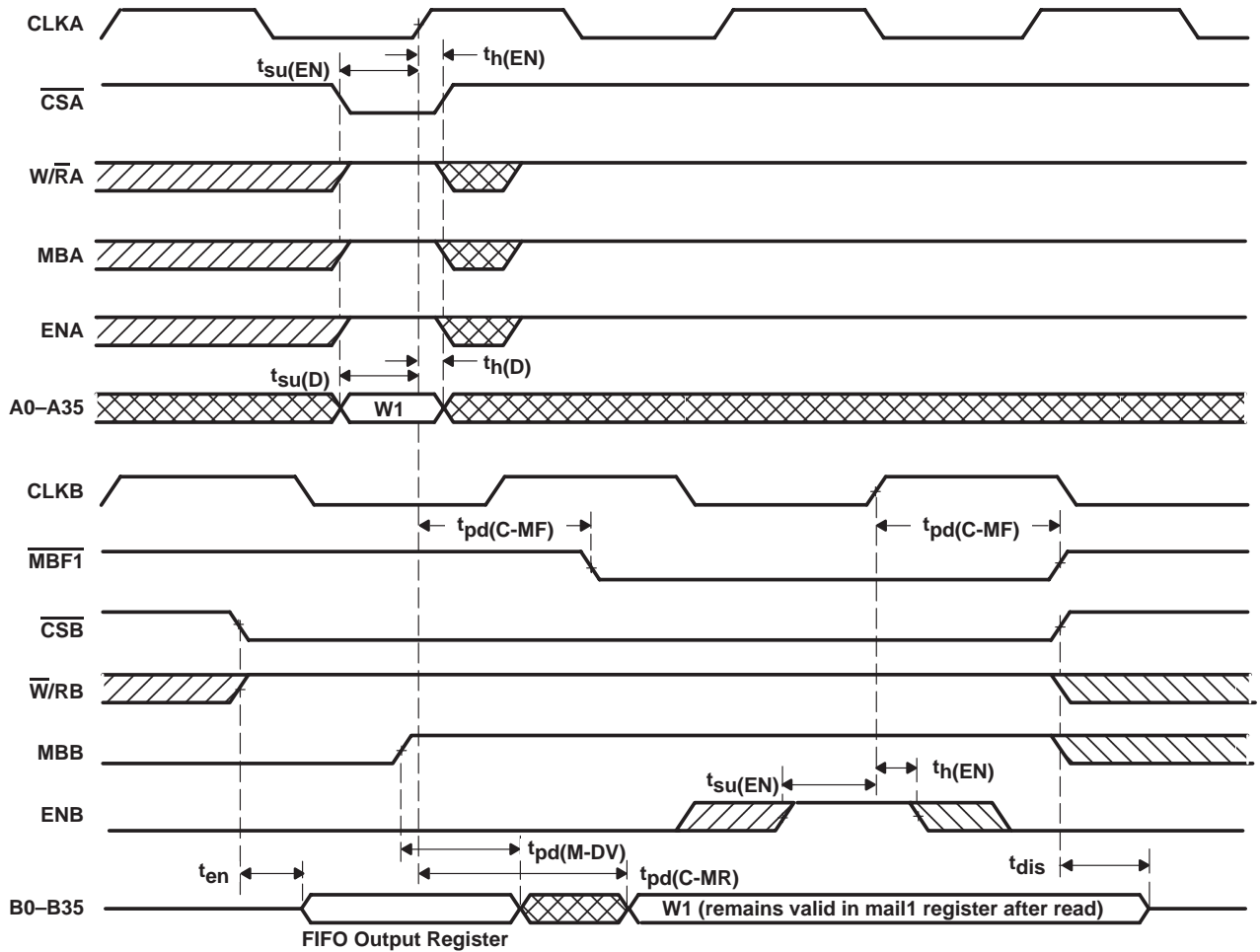
Figure 14. Mail1 Register and \overline{MBF1} Flag
