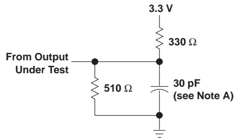
LOAD CIRCUIT
