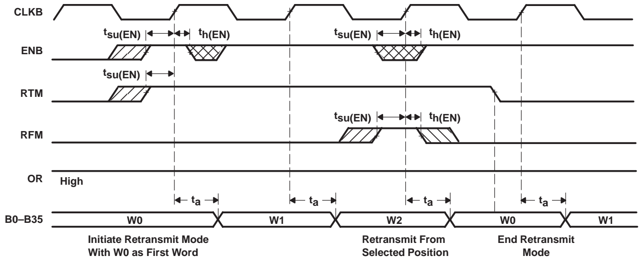
Figure 10. Retransmit Timing Showing Minimum Retransmit Length
