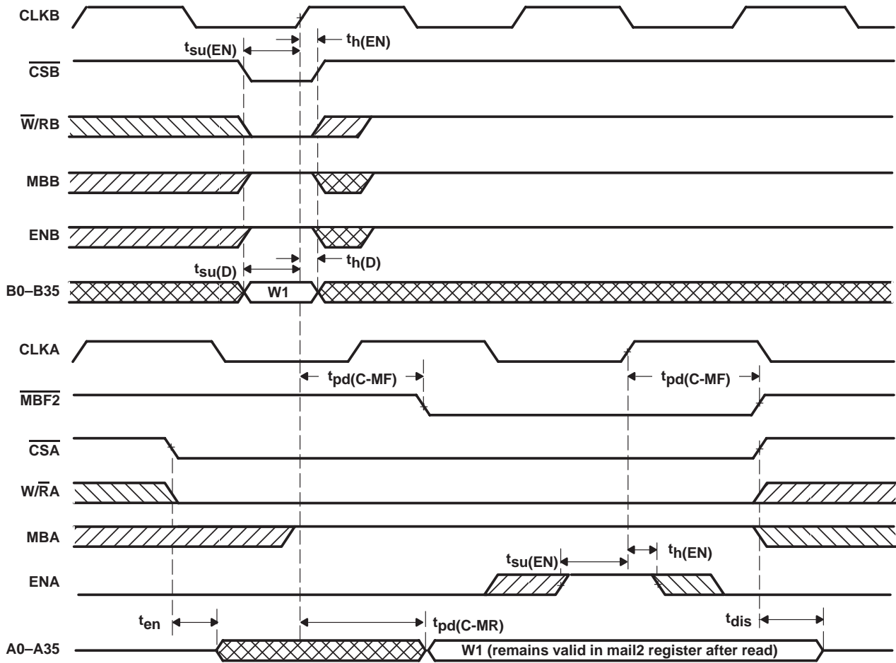
Figure 15. Mail2 Register and \overline{\text{MBF2}} Flag
