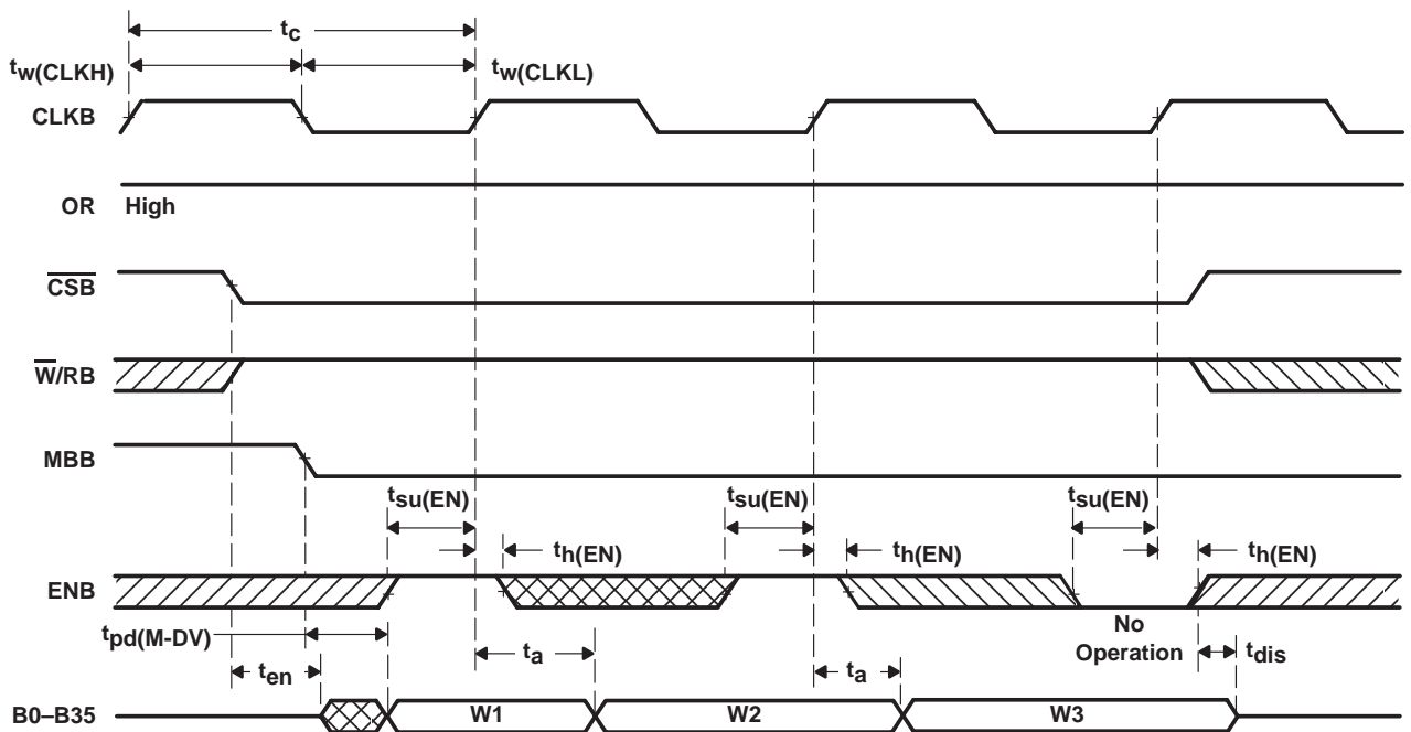
Figure 5. FIFO Read Cycle
