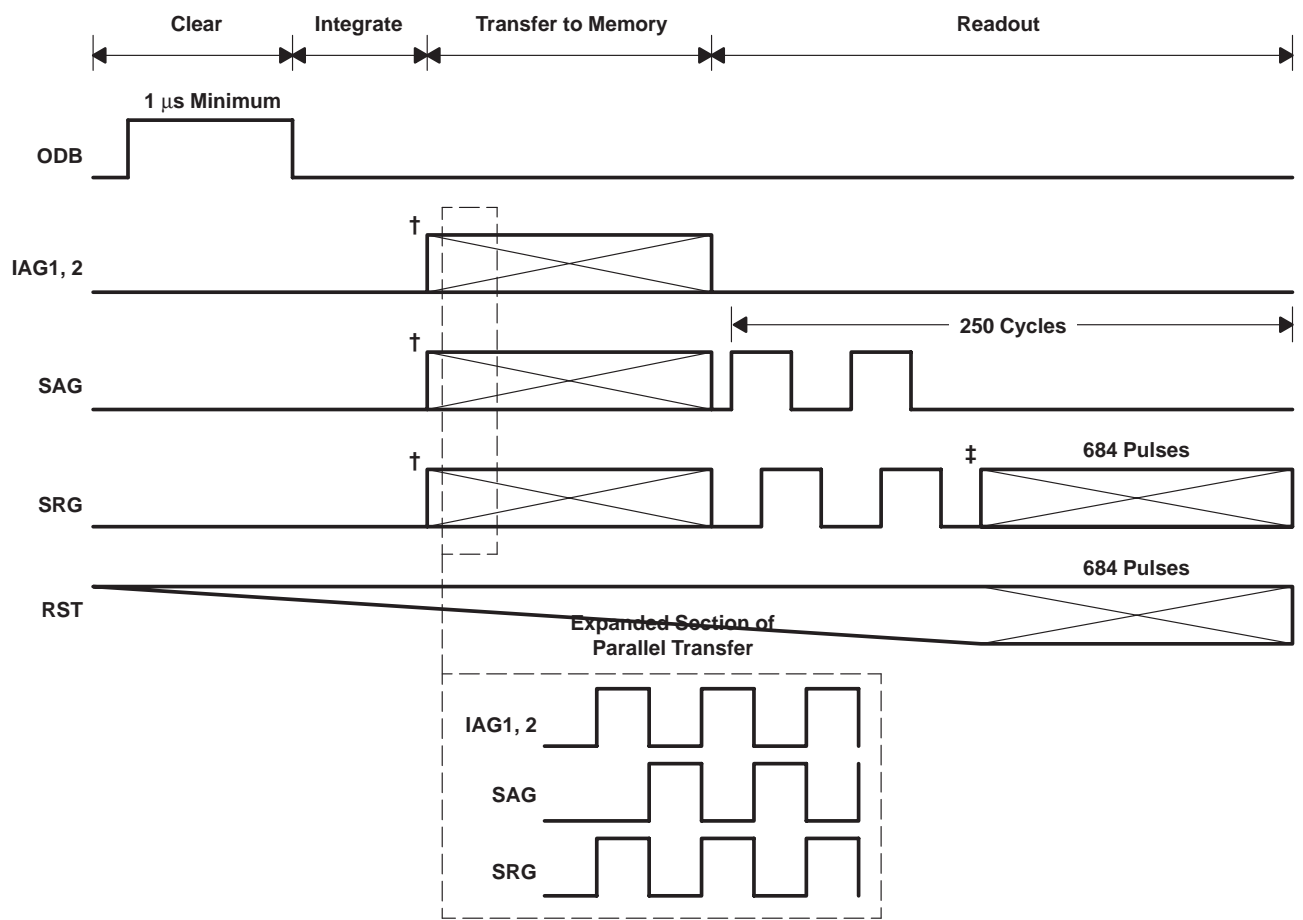
Figure 3. Interlace Timing
