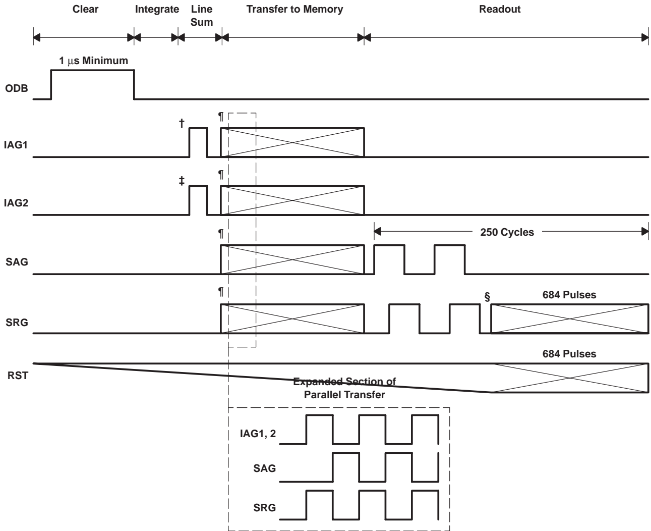
Figure 6. Line-Summing Timing
