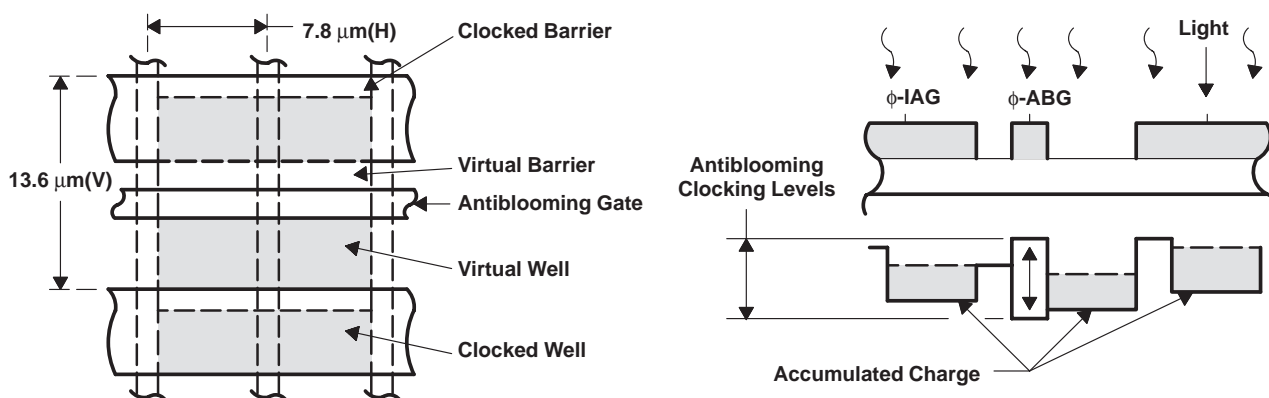
Figure 1. Charge-Accumulation Process
