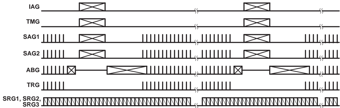
Figure 7. Vertical Timing, Low-Light Mode
