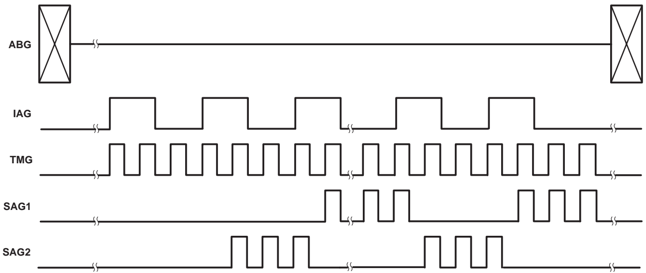
Figure 10. Parallel-Transfer Timing
