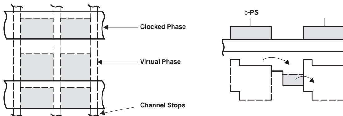
Figure 2. Charge-Transfer Process
