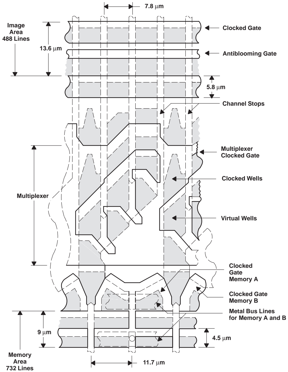
Figure 3. Layout of Multiplexing Gate
