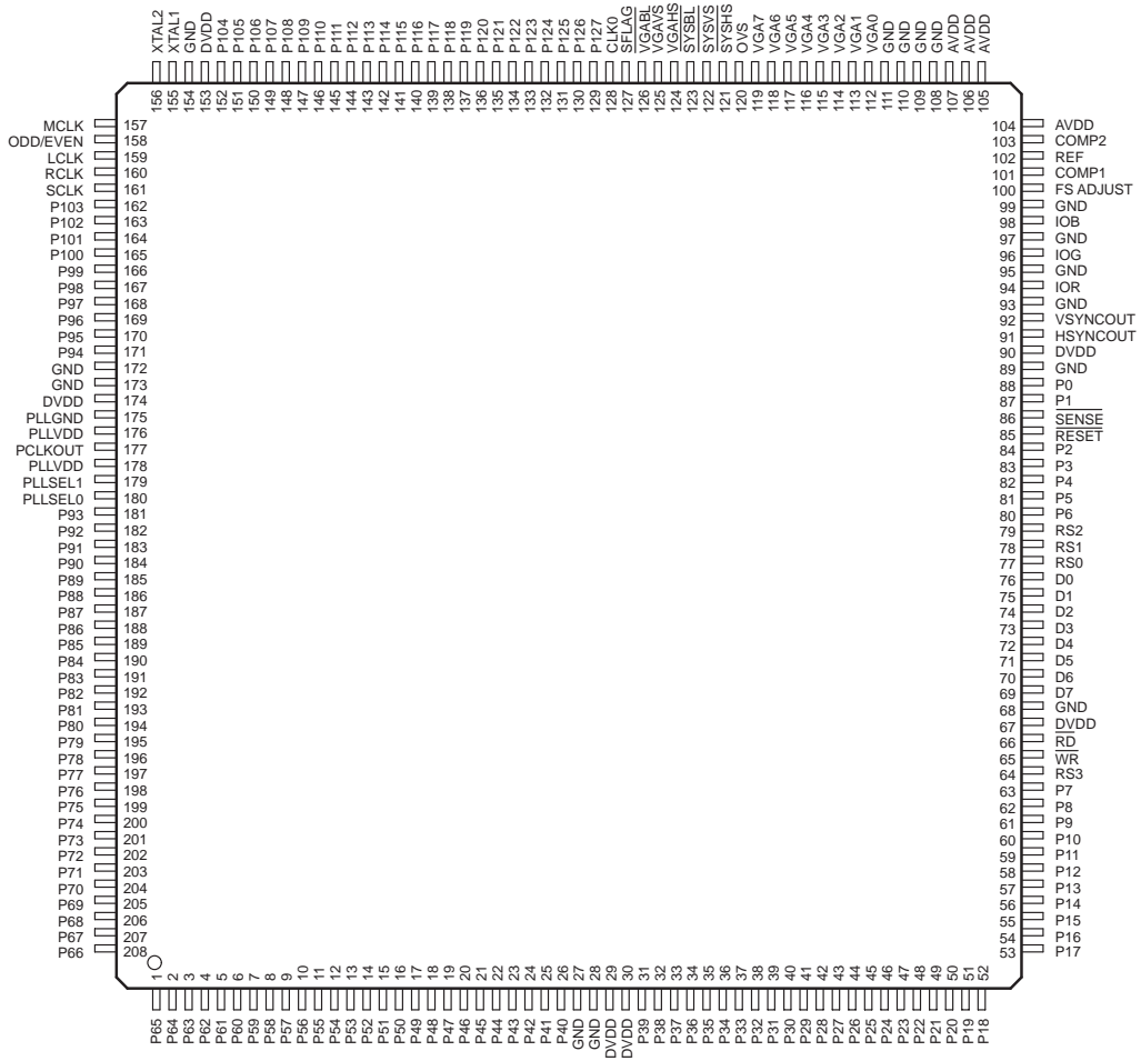
Figure 1–2. Terminal Assignments
