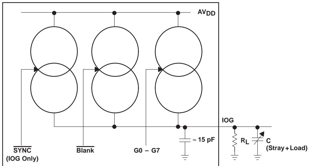
Figure 2-12. Equivalent Circuit of the Current Output (IOG)
