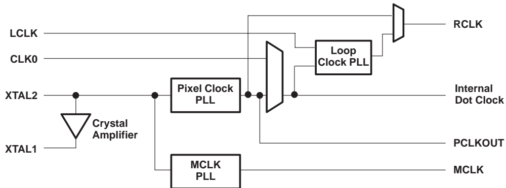
Figure 2-1. TVP3030 Clocking Scheme
