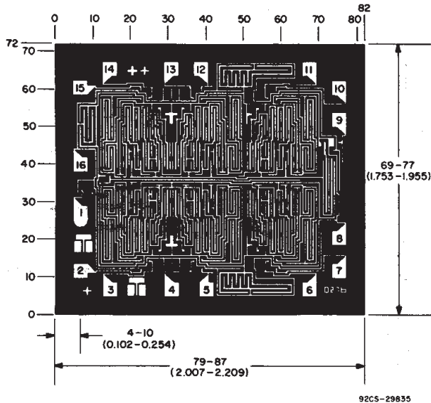
Dimensions and pad layout for CD40174B.
