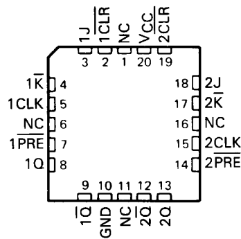
SN54HC109 . . . FK PACKAGE (TOP VIEW)
