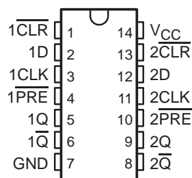
SN54LV74A . . . J OR W PACKAGE SN74LV74A . . . D, DB, DGV, NS, OR PW PACKAGE (TOP VIEW)
