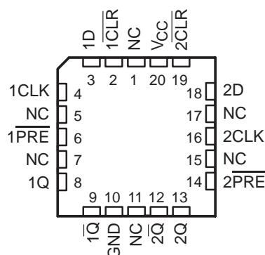
SN54LV74A . . . FK PACKAGE (TOP VIEW)
