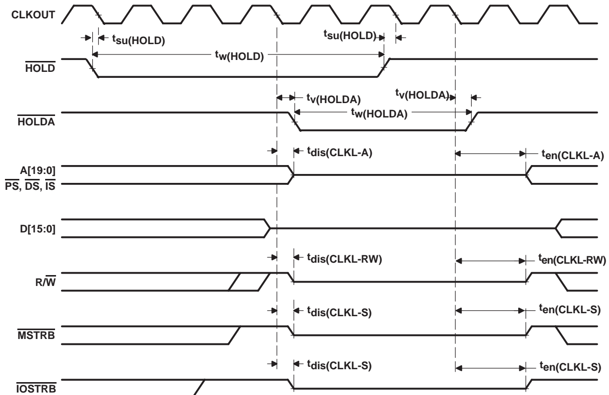
Figure 20. \overline{HOLD} and \overline{HOLDA} Timings (HM = 1)
