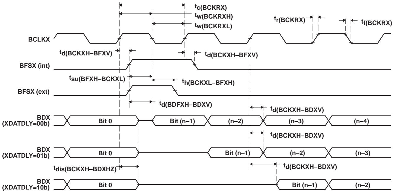
Figure 28. McBSP Transmit Timings
