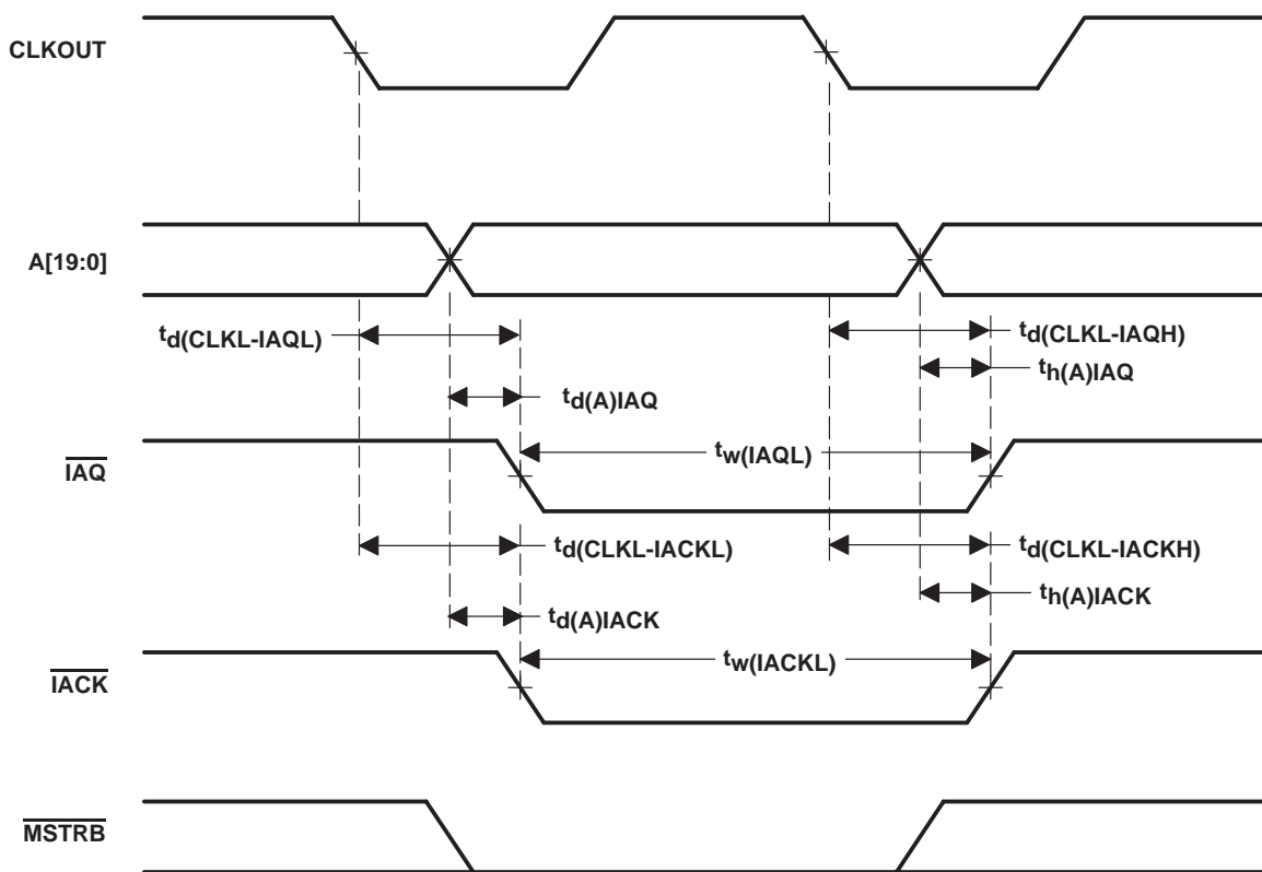
Figure 24. \overline{\text{IAQ}} and \overline{\text{IACK}} Timings
