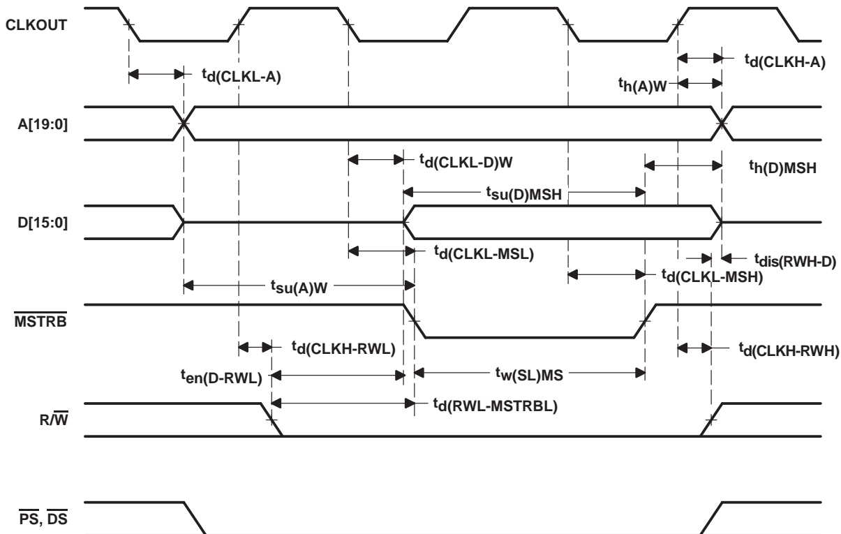
Figure 13. Memory Write ( \overline{\text{MSTRB}} = 0 )
