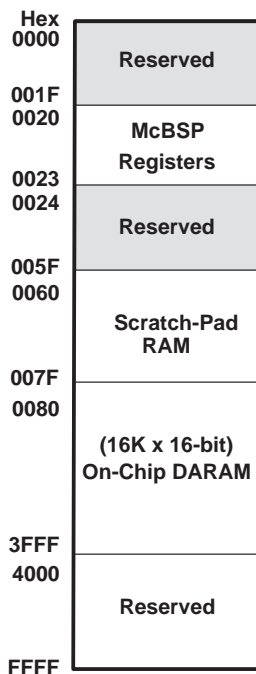
Figure 6. '5402 DMA Memory Map
