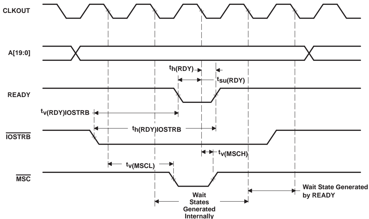
Figure 18. I/O Read With Externally Generated Wait States
