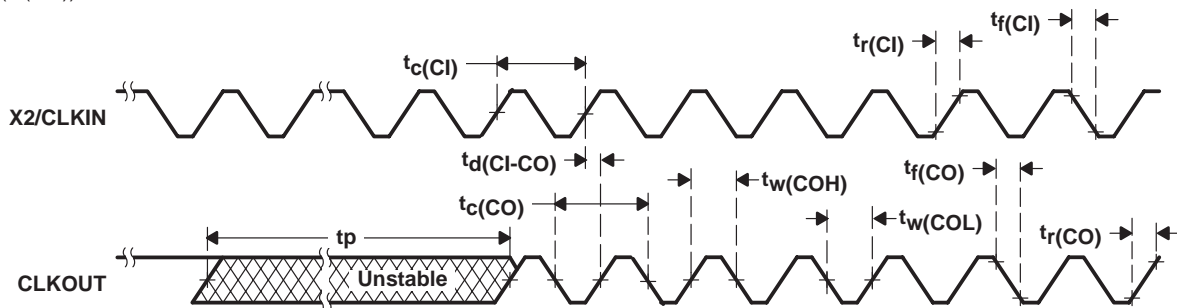
Figure 11. External Multiply-by-One Clock Timing
