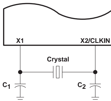
Figure 9. Internal Oscillator With External Crystal
