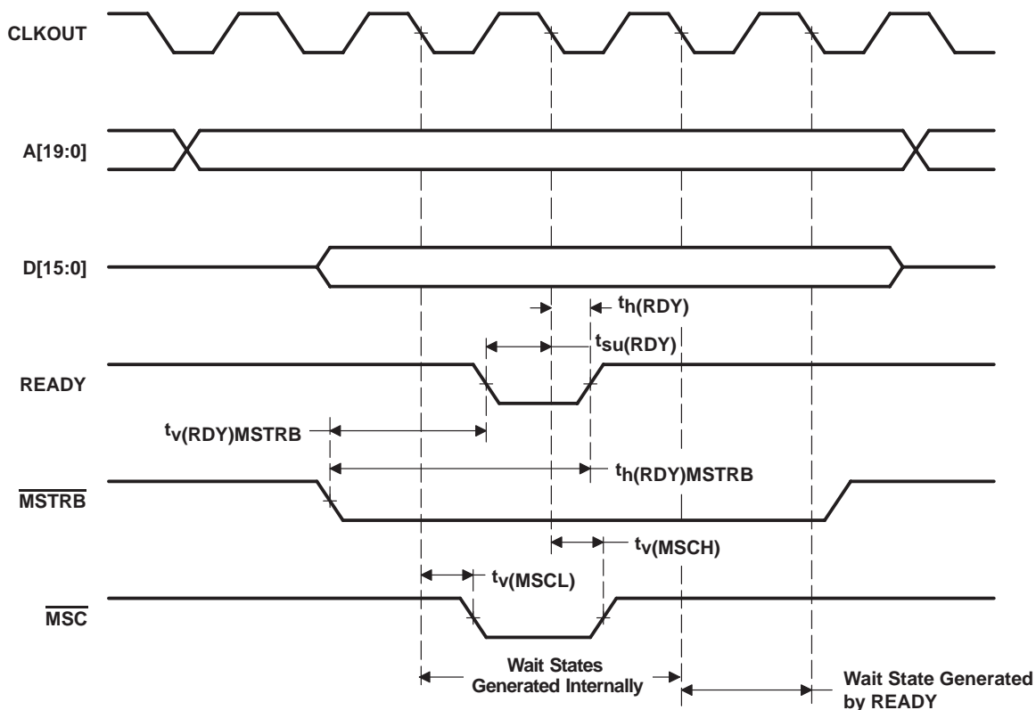
Figure 17. Memory Write With Externally Generated Wait States
