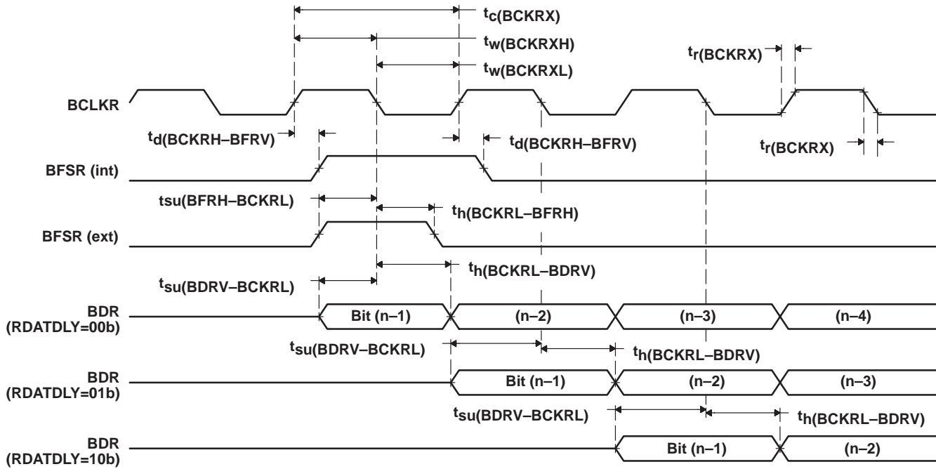
Figure 27. McBSP Receive Timings
