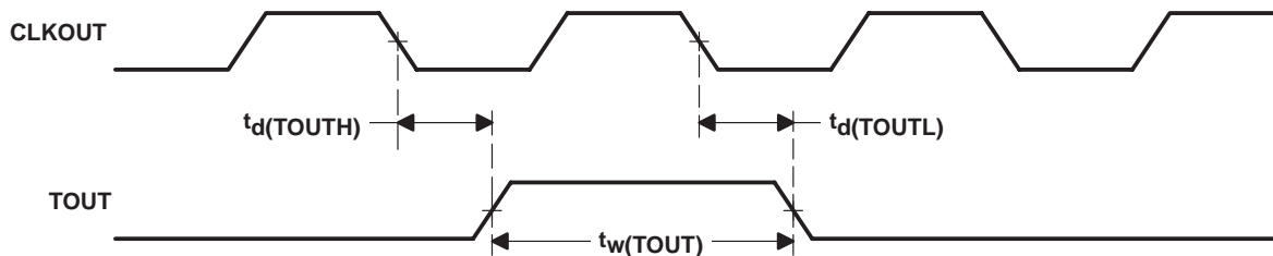
Figure 26. TOUT Timing
