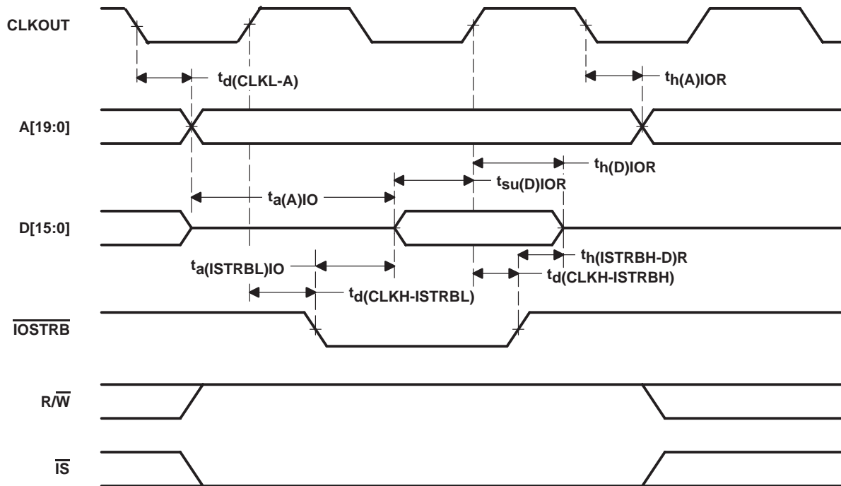
Figure 14. Parallel I/O Port Read ( \overline{IOSTRB} = 0 )
