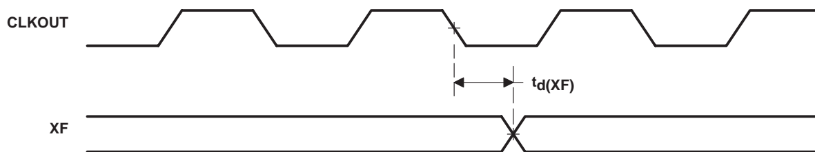
Figure 25. XF Timing
