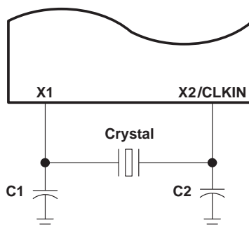
Figure 4. Internal Clock Option
