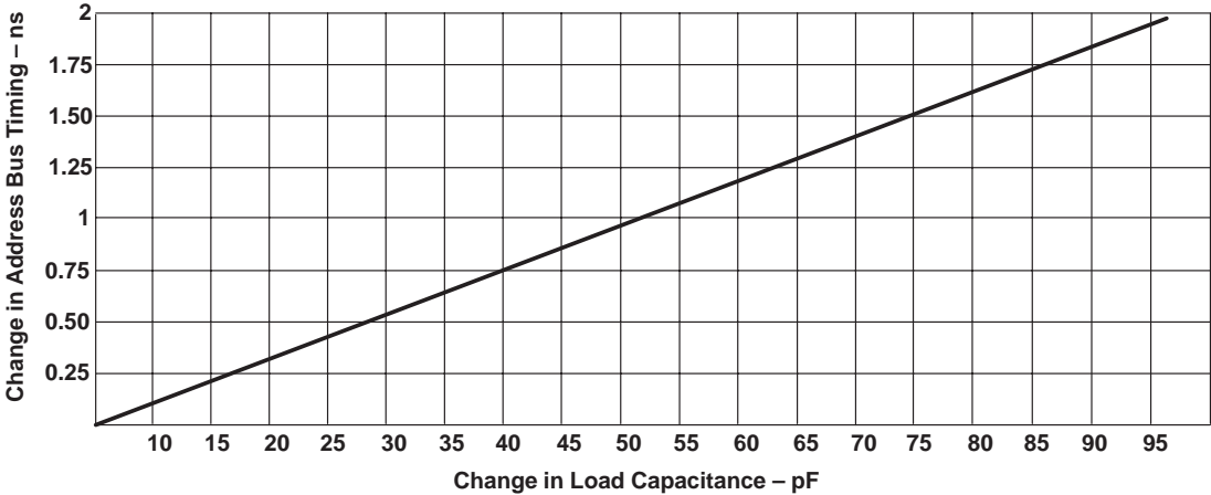
Figure 8. Address Bus Timing Variation With Load Capacitance
