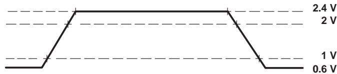
Figure 2. TTL-Level Outputs
