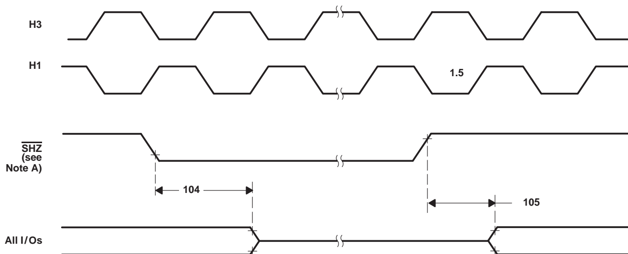
Figure 30. Timing for SHZ
