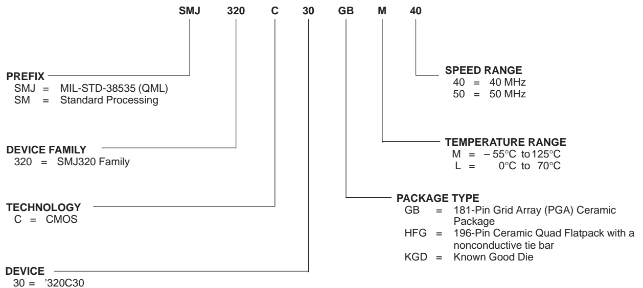
Figure 31. SMJ320C30 Device Nomenclature
