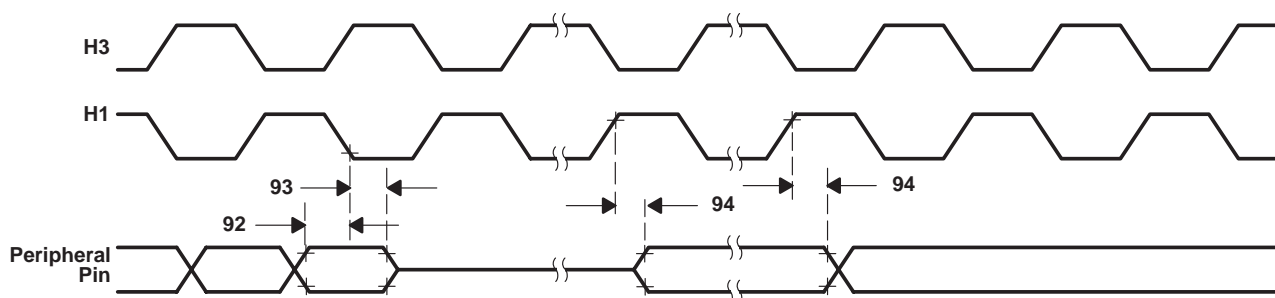
Figure 26. Timing for Peripheral Pin General-Purpose I/O
