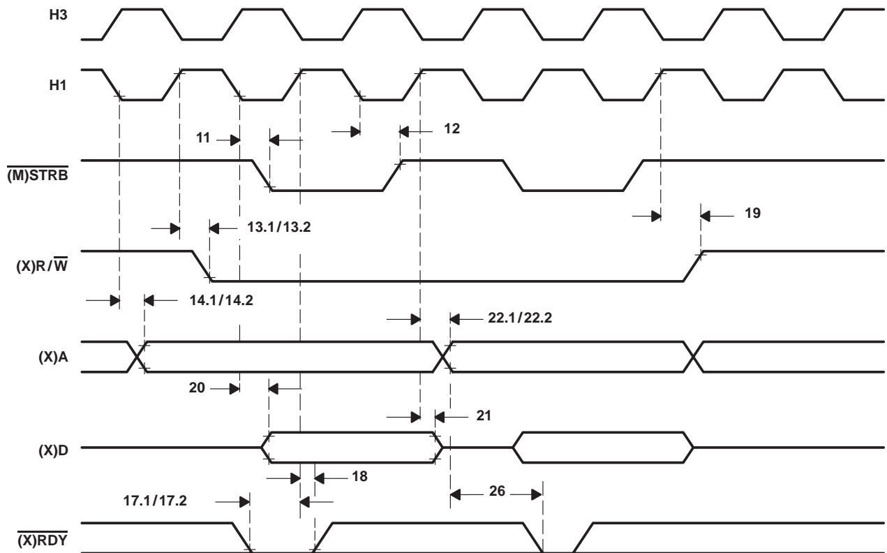
Figure 11. Timing for Memory [(M)STRB = 0] Write
