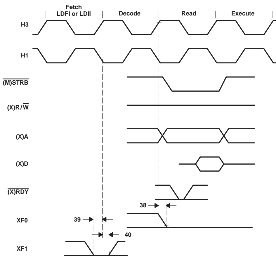
Figure 14. Timing for XF0 and XF1 When Executing LDFI or LDII
