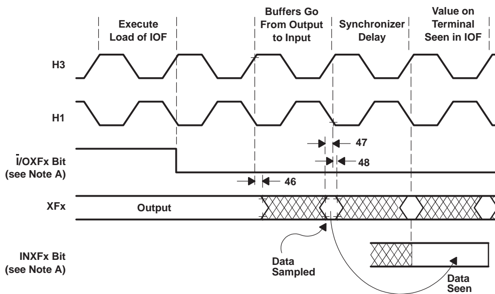
Figure 18. Timing for Change of XF x From Output to Input Mode
