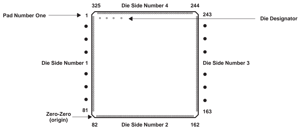
Figure 2. '320C40 Die Numbering Format (See Table 1)
