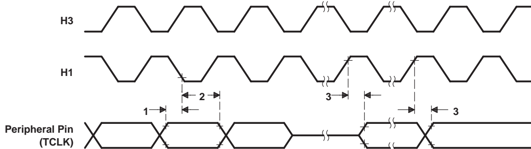
Figure 27. Timer Pin Timing Cycle
