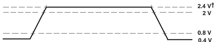
Figure 7. TTL-Level Inputs
