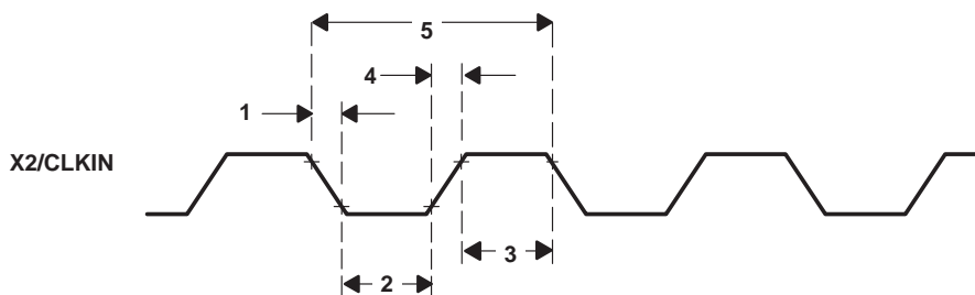
Figure 8. X2/CLKIN Timing
