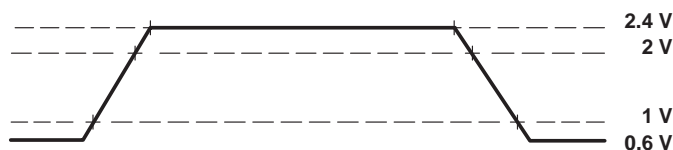
Figure 6. TTL-Level Outputs
