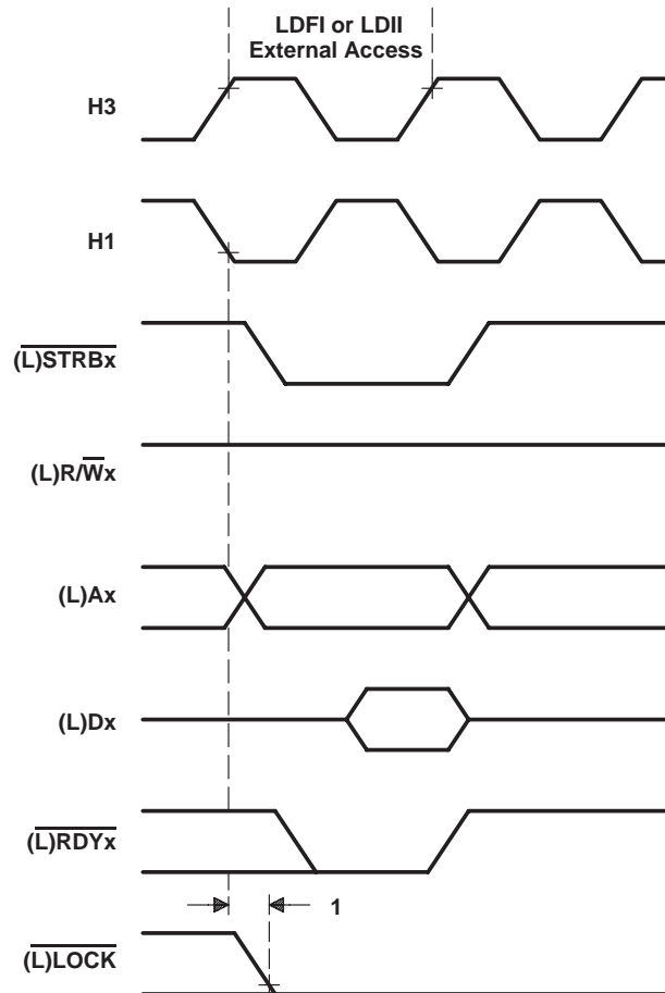
Figure 13. Timing for (L)LOCK When Executing LDFI or LDII
