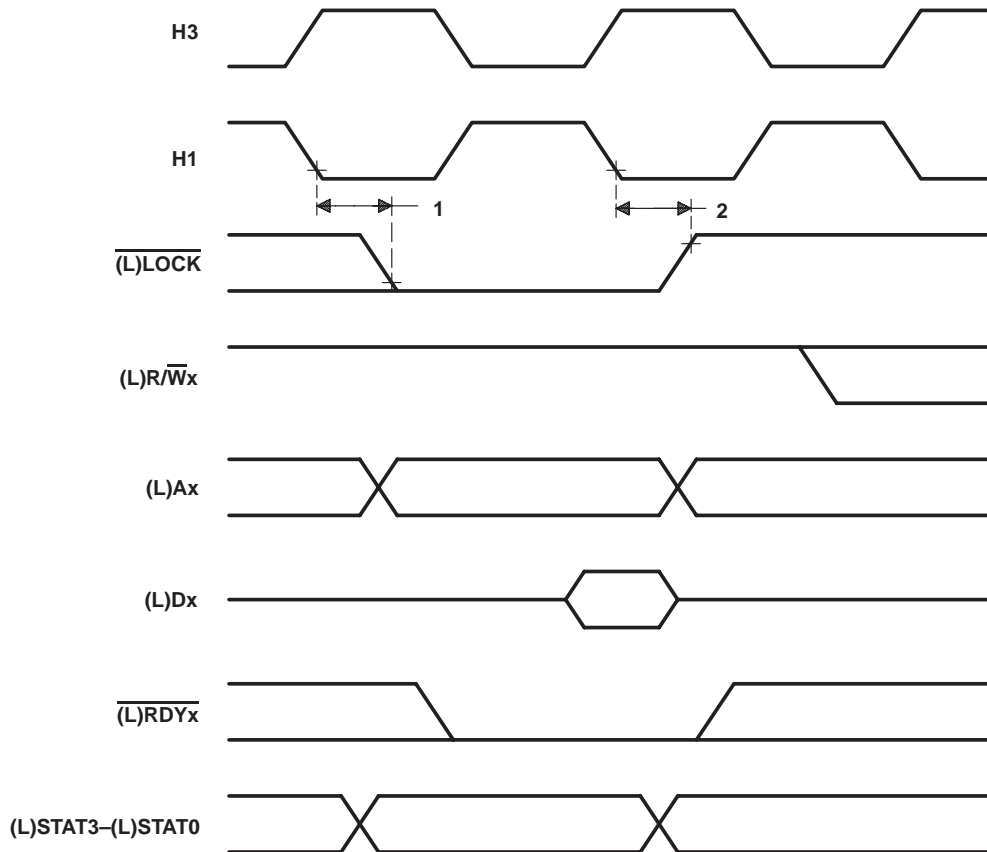
Figure 15. Timing for \overline{\text{(L)}}\text{LOCK} When Executing SIGI
