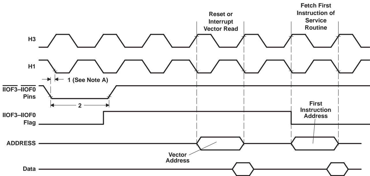
Figure 21. \overline{\text{IIOF3}}\text{--}\overline{\text{IIOF0}} Interrupt Response Timing [ P=t_{c(H)} ]
