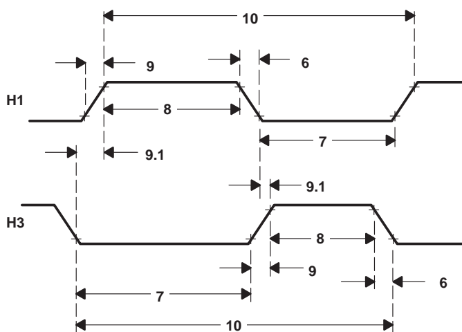
Figure 9. H1/H3 Timings
