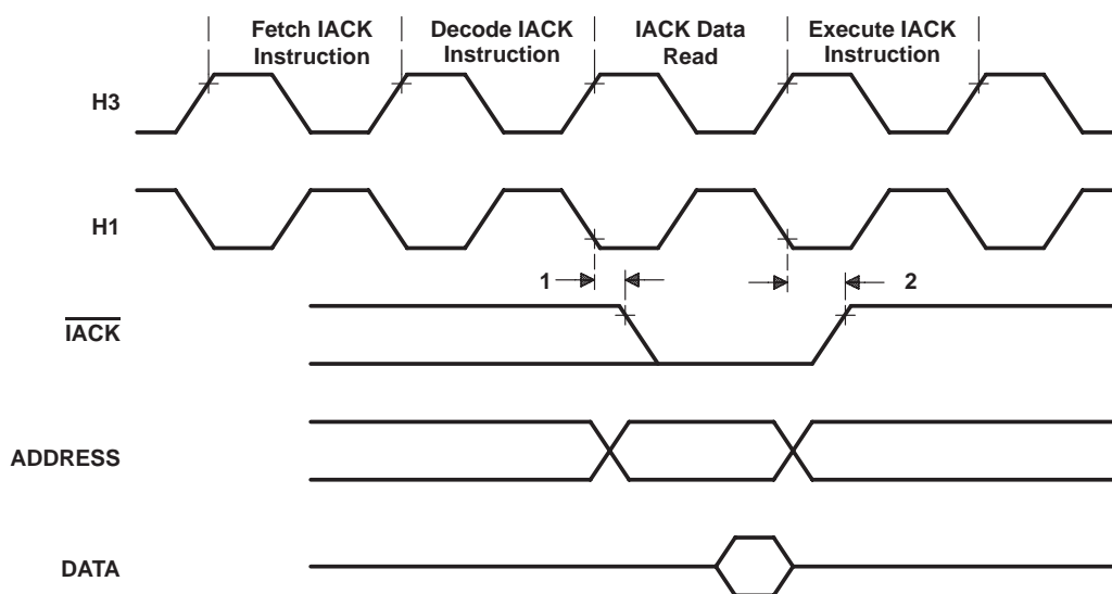
Figure 22. \overline{\text{IACK}} Timing
