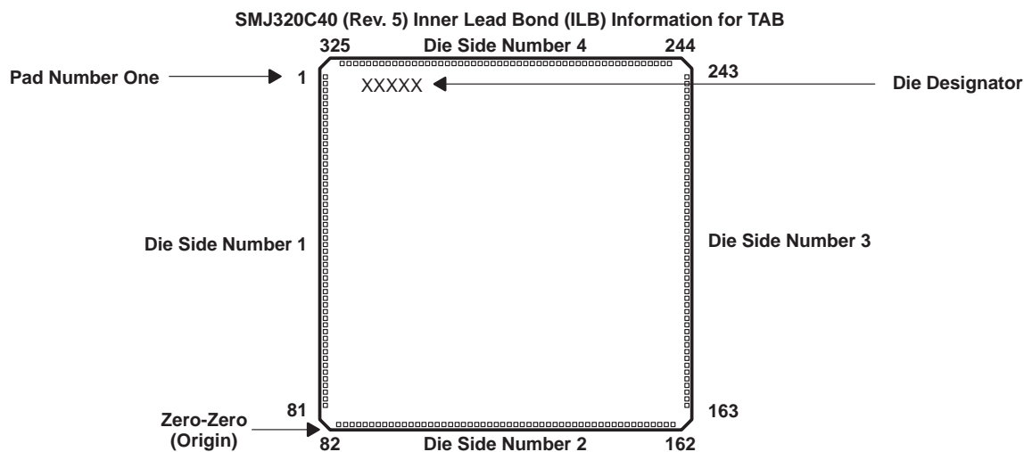
Figure 4. SMJ320C40 Die Numbering Format (See Table 2)
