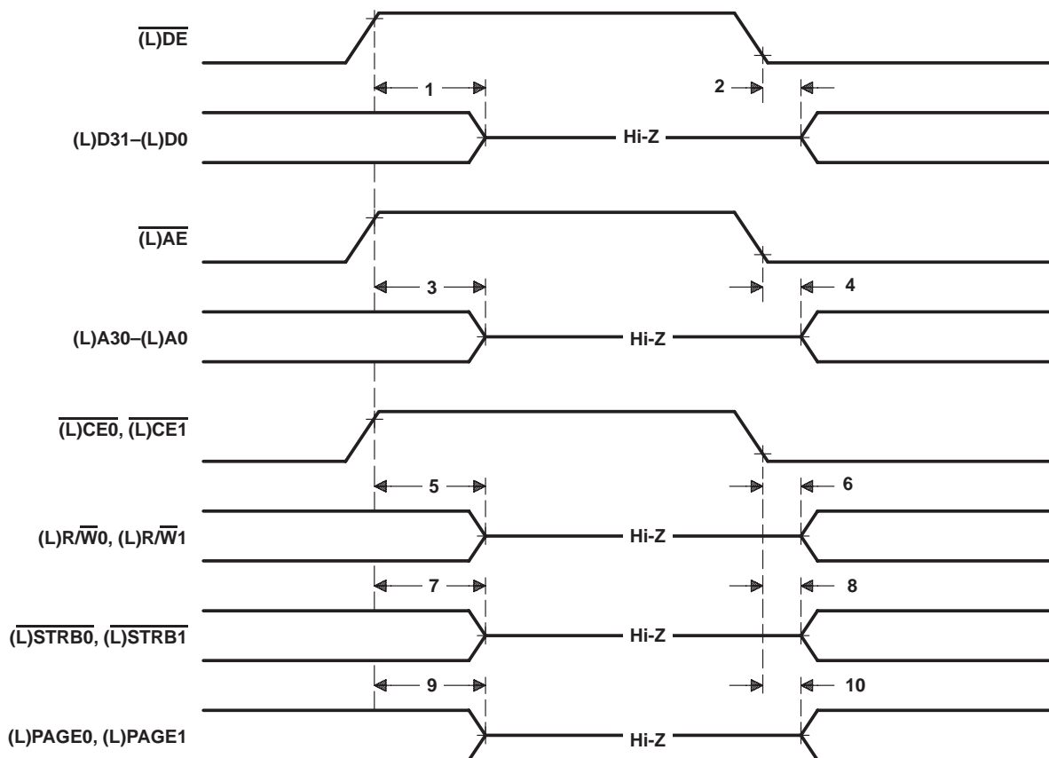
Figure 12. (L)DE, (L)AE, and (L)CEx Enable Timings
