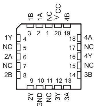
SN54ALS1000A, SN54AS1000A ... FK PACKAGE (TOP VIEW)
