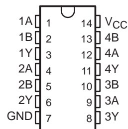
SN54ALS1000A, SN54AS1000A ... J PACKAGE SN74ALS1000A, SN74AS1000A ... D OR N PACKAGE (TOP VIEW)
